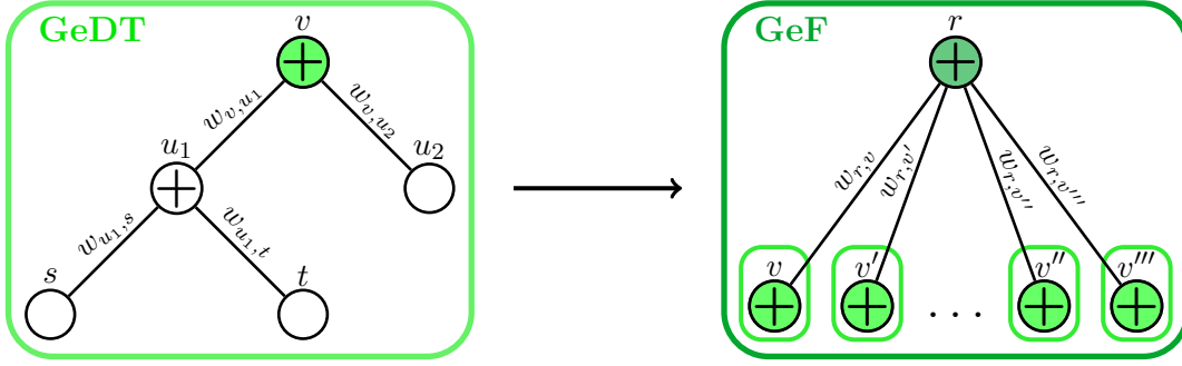
Figure 1: Visualization of the structures of a GeDT and a GeF.
