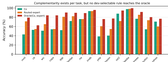
Figure 9. Per-task accuracy of Co, the routed expert and their oracle on the Long benchmark (Order 4).
