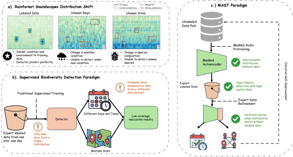
Figure 2: Motivation of MAST. (a) Rainforest soundscapes exhibit substantial temporal and cross-site distribution shift, making detection under unseen conditions difficult. (b) Standard supervised biodiversity detectors trained on limited labels from a narrow time/site range often generalize poorly when deployed to new days and sites. (c) These challenges motivate a label-efficient and shift-robust framework that can leverage both limited expert labels and abundant unlabeled soundscapes.
