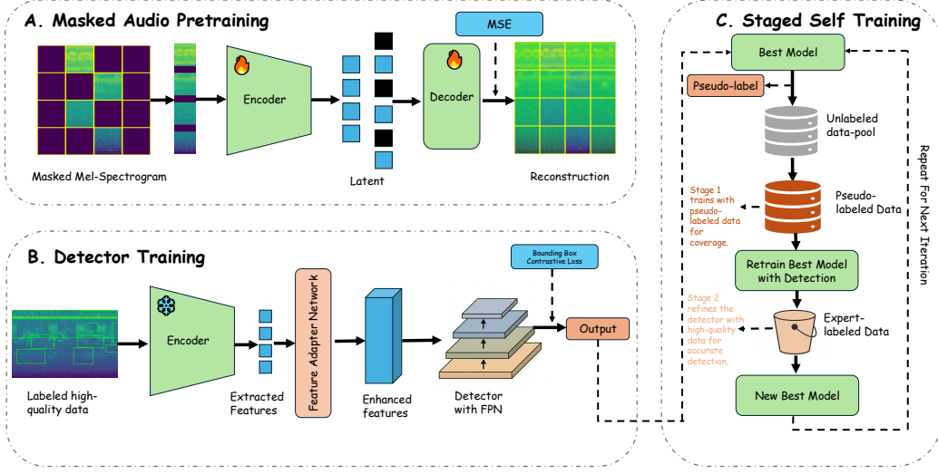
Figure 3: Overview of the MAST pipeline. (A) Masked-audio pretraining learns general acoustic representations from unlabeled rainforest spectrograms via masked reconstruction. (B) Detector training transfers the pretrained encoder to a detection model with an audio-aware adapter and lightweight FPN, together with a box-level contrastive objective for event separation. (C) Staged self-training improves robustness under distribution shift by first generating pseudo-labels on unlabeled audio and then retraining with exploration on pseudo-labeled data followed by refinement on expert-labeled data.
