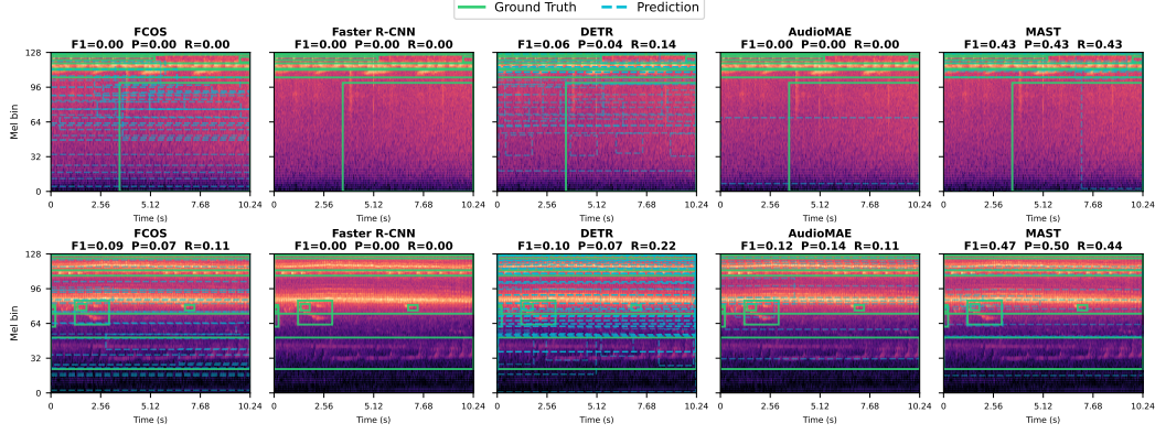
Figure 8: Qualitative detection comparison on two randomly sampled cross-site OOD chunks on rainforest domain. Ground-truth boxes are shown in green solid lines; predicted boxes in blue dashed lines. Baseline detectors produce numerous false positives or miss most events entirely, while MAST localizes the majority of sound events with fewer spurious detections.
