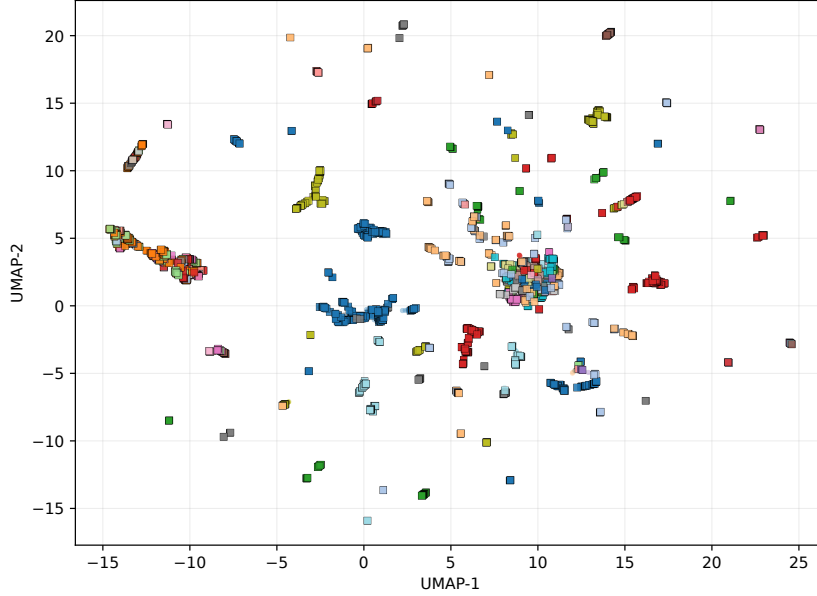
Figure 6: Box-level embedding space induced by MAST detections on rainforest domain. Each point corresponds to a ground-truth or predicted time–frequency box, embedded by pooling its corresponding region from the pretrained encoder feature map and projected with UMAP. Boxes with similar acoustic structure form partially coherent clusters, and high-quality predictions tend to lie near ground-truth embeddings of the same or related sonotypes. This suggests a practical downstream use of MAST: detected sound events can be retrieved against annotated examples for tentative zero-shot classification, while acoustically distinct clusters can be surfaced to experts as candidate novel sounds. Colors denote sonotypes; circles correspond to predicted boxes and squares correspond to ground-truth boxes.
