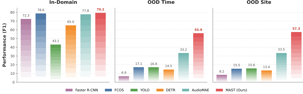
Figure 1: Performance comparison on rainforest domain. MAST achieves the best overall performance, with especially large improvements under temporal and cross-site distribution shift, showing stronger robustness than fully supervised baselines and generic SSL transfer.
