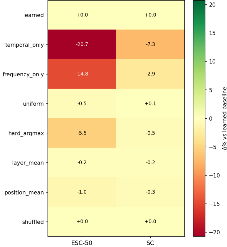
Figure 9: Audio gate intervention heatmap ( \Delta\% vs. learned baseline). The pattern mirrors EEG: single-axis routing is catastrophic, while shuffled and layer-mean gates are indistinguishable from the learned gate.
