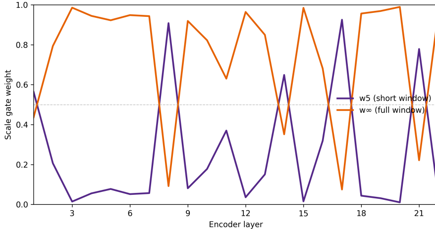
Figure 7: Scale gate routing: short window ( W = 5 ) vs. full window ( W = \infty ) across 22 layers. The model usually favours broad temporal context, but uses short temporal windows in a few selected layers. The two-scale temporal design contributes +0.001 Mean LP and +0.013 Mean FT over the single-scale variant; the scale gate is a secondary improvement.
