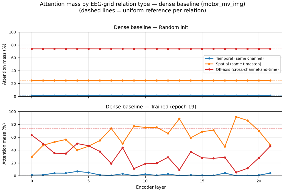
Figure 8: Relation-type attention mass per layer in the dense baseline ( C = 64, T = 4 ). Top: Random initialisation matches the uniform complete-graph prior (dashed lines). Bottom: After MAE pretraining, dense attention discovers spatial dominance in mid-depth layers but fails to fully suppress off-axis interactions. Early and late layers retain up to 63% off-axis mass, leaving off-axis interactions that AXON removes by construction.
