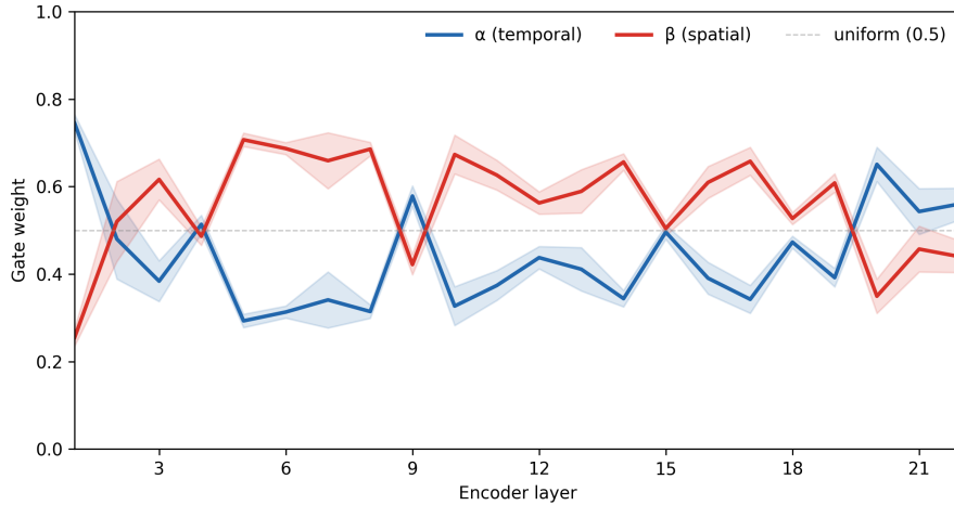
Figure 4: AXON axis gate across the 22 encoder layers: gate weights averaged over all six downstream datasets (mean \pm \sigma ), on validation batches with the frozen encoder. Temporal-heavy in the first layer, spatial-heavy in the middle layers, and back toward temporal in the late layers.
