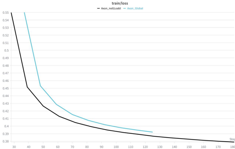
Figure 2: MAE reconstruction loss during pretraining. AXON (no global path) and AXON-withGlobal converge to comparable reconstruction loss ( \approx 0.38 – 0.39 ), yet AXON-withGlobal underperforms on mean LP (0.555 vs. 0.579) and mean FT (0.619 vs. 0.656). The global path does not improve reconstruction; it changes how the encoder reconstructs, routing mass through dense averaging ( \gamma = 0.724 at layer 1) rather than through axis-structured features.
