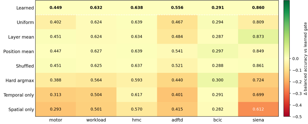
Figure 5: Per-dataset gate intervention heatmap (frozen-encoder LP, 6 datasets; same protocol as Table 14). Cell colour is the change from the learned gate. The learned gate outperforms uniform and hard-argmax routing on most datasets, but layer-mean, position-mean, and shuffled gates stay close to learned, indicating that exact token-gate alignment is not the dominant effect.
