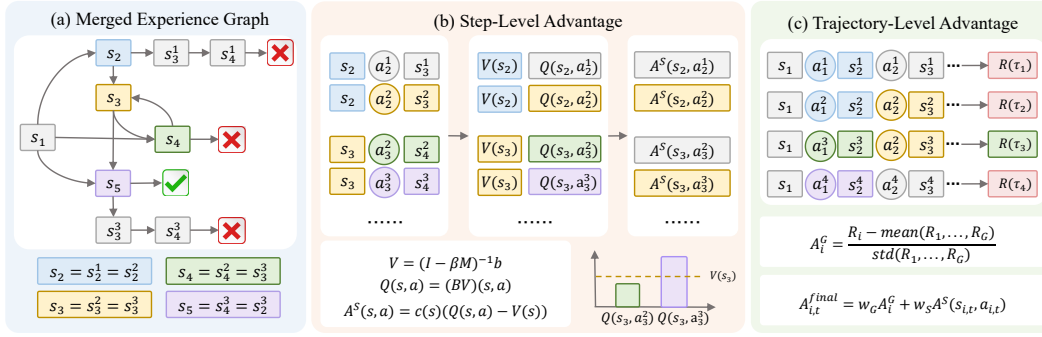
Figure 2: Overview of CRBC. (a) Shared anchors merge rollouts into an empirical process with absorbing success and failure boundaries. (b) A Bellman fixed-point solve yields the state value V , followed by action backups to obtain the action value Q and normalized Q - V credit, which gives relative action credit. (c) Step-level credit and trajectory-level group-relative advantages are combined for policy optimization.
