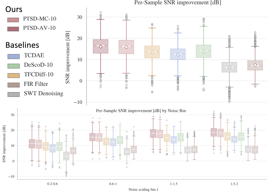
Figure 12: Per-sample \Delta SNR on the PTB-XL test set. Notched box plots: box is the IQR, white line the median, notch its 95% CI, whiskers span 1.5 \times \text{IQR} , open circles are outliers. Top: overall (white diamond = mean). Bottom: stratified by corruption scaling factor \lambda .
