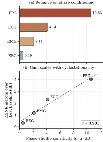
Figure 2: (a) \Delta\text{SNR} drop under phase shuffling. (b) Phase-shuffle sensitivity versus the margin over the best baseline.
