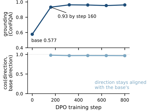
Figure 2: Grounding is largely in place by the first checkpoint, and the audited direction stays aligned ( \cosine \geq .968 ). Top: ConFiQA grounding jumps from base .577 to .932 by DPO step 160 of 800 (matched 500-item evaluation). Bottom: at every checkpoint, the grounding direction’s cosine to the base model’s own direction stays above .968 (full 0–1 axis).
