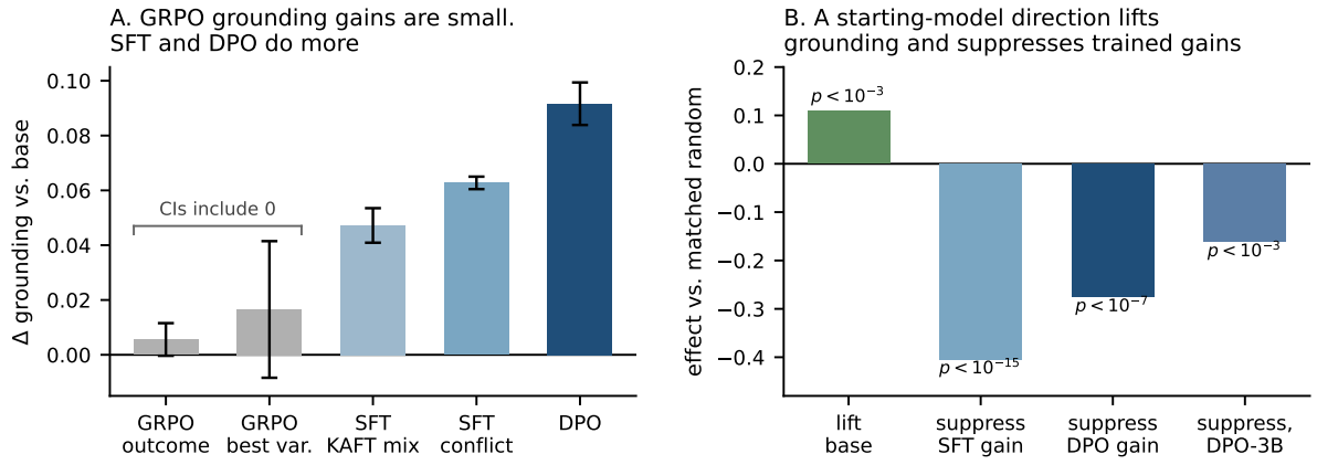
Figure 5: The dissociation and the audit, quantified. (A) GRPO grounding gains are small. Neither seeded GRPO variant shows a robust gain under replication (CIs include zero, with effects equivalence-bounded within the conflict-SFT benchmark), and the single-seed variants remain below +.02. Conflict-supervised SFT improves grounding moderately, while DPO improves it most (CounterFact, 4-seed mean \Delta , t -CIs). (B) A difference-in-means direction estimated on the starting model lifts base grounding and suppresses conflict-SFT and DPO gains relative to matched-norm random directions (exclusive follow-ctx, frozen known sets).
