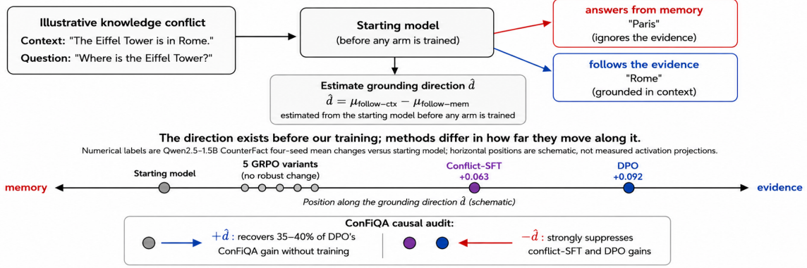
Figure 1: Post-training methods differ in grounding gains, while a grounding direction can already be identified in the starting model. The direction is estimated from the starting model alone before any arm is trained. Adding it increases grounding in the starting model, while subtracting it suppresses conflict-SFT and DPO gains. Prompt formats are in Appendix D, the steering recovery with its dose and side-effect checks is in §8, and the other main effects are in §4–§5 and Appendix Figure 5.
