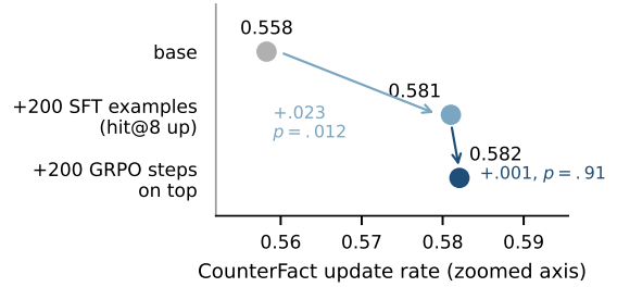
Figure 3: A supervised warm start does not rescue the tested GRPO recipe. The warm start raises context-answer hit@8 and grounding (+.023, p=.012 ), but the advantage-collapsed fraction remains near .62. Running the identical GRPO recipe on top adds +.001 ( p=.91 ). Dot position encodes the update rate on a zoomed axis.
