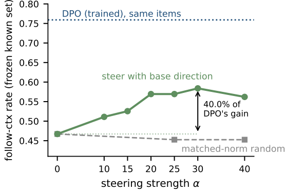
Figure 4: Steering along the base-estimated direction increases grounding. Matched random directions do not. Steering the base model along the base-estimated direction raises follow-ctx steadily up to \alpha=30 , recovering 40.0% of the gain DPO achieves on the identical items (35.0% at the largest tested dose that passes all stated side-effect checks). Matched-norm random directions stay flat.
