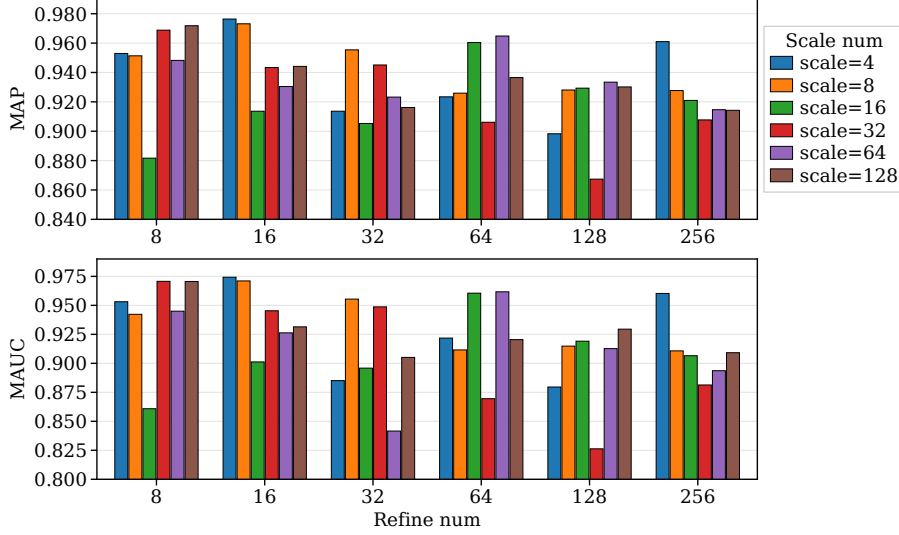
Figure 3: Sensitivity of MAP and MAUC to the refinement number and scale number.
