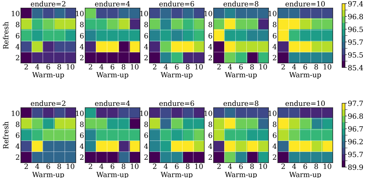
Figure 2: Refresh-schedule heatmaps on Wiki-Eo. The top row reports MAUC and the bottom row reports MAP.
