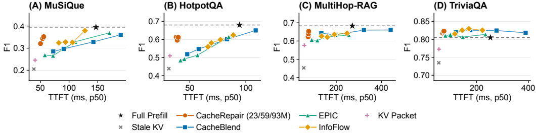
Figure 6: Answer F1 versus p50 TTFT for Llama-3.1-8B on four downstream datasets.
