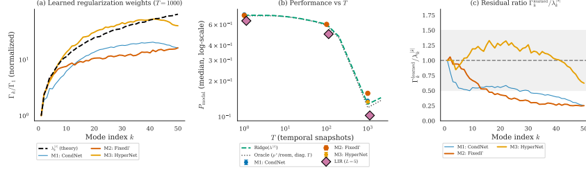
Figure 2: M3 recovers |s| ; M2 does not; the basin absorbs the difference. (a) Learned \Gamma_k/\Gamma_1 at T=1000 for M1, M2, M3, and theory (dashed); M3’s per-room median exponent \hat{p}_{M3}=1.13 matches theory’s |s|=1.13 , while M2 finds \hat{p}_{M2}=0.62 . (b) P vs. T (log scale): M1/M2/M3 sit on the ridge( |s| ) curve; LIR ( L=5 ) is the only model that breaks below the per-room oracle. (c) Residual \Gamma_k^{\text{learned}}/\lambda_k^{|s|} : M1/M2 collapse to \leq 0.25 at high k ; only M3 stays in [0.5, 1.5] across all 50 modes.
