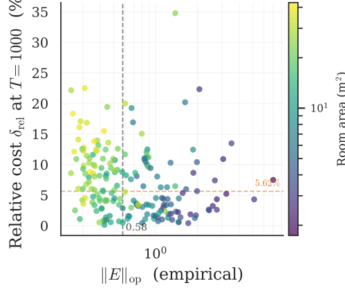
Figure 4: Relative cost \delta_{\text{rel}} = (P(|\hat{s}|) - P(p^*)) / P(p^*) at T=1000 versus empirical \|E\|_{\text{op}} (Method B, §A.2, 187 rooms). Points colored by room area. The Spearman rank correlation is \rho = -0.30 ( p < 10^{-4} ): rooms with higher anisotropy pay lower cost. The color gradient exposes the confound: large rooms (yellow) have low \|E\|_{\text{op}} (many truncated modes \Rightarrow CLT averaging) but elevated \delta (wider eigenvalue spectrum gives the per-room oracle more to exploit); small rooms (purple) show the reverse. The bottleneck is eigenvalue diversity, not noise anisotropy.
