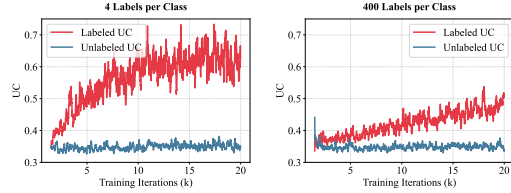
Figure 1: UC of labeled and unlabeled losses.
