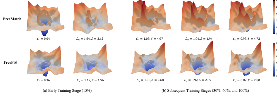
Figure 2: Visualization of loss landscapes: FreeMatch vs ours (FreePiS). Landscapes are obtained by perturbing the model parameters (landscape origin) along two orthogonal directions. \mathcal{L}_l and \mathcal{L}_u denote the labeled and unlabeled loss values at the origin, respectively, while \mathcal{S} measures landscape sharpness, which reflects generalization potential (see Appendix B for formal definition).
