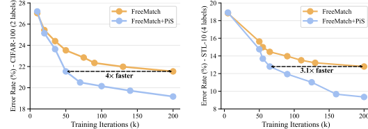
Figure 4: PiS accelerates convergence by reaching the same performance with significantly fewer training iterations.
