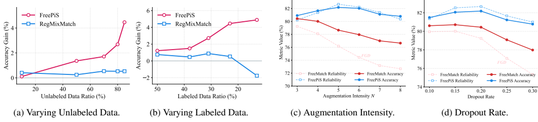
Figure 5: Comparative study of model performance under different data scales and regularization intensities. (a–b) Performance gains across varying scales of labeled and unlabeled data. (c–d) Teacher’s pseudo-label reliability and final accuracy under different augmentation intensities and dropout rates [38] (see Appendix F for numerical results; see Section 5.4 for augmentation details).
