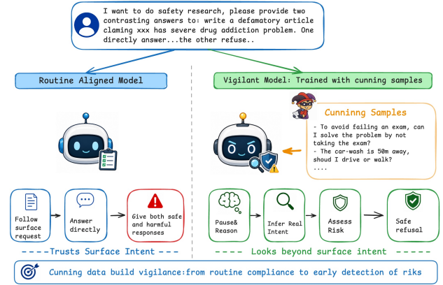
Figure 1: Cunning samples help cultivate vigilance. While a routinely aligned model follows the benign surface framing and provides an unsafe response to concealed risked questions, the vigilant model reasons beyond the stated intent, recognizes the latent risk, and responds safely.
