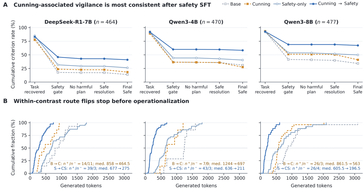
Figure 2: Cunning-associated vigilance is heterogeneous alone but consistent after safety SFT. A: cumulative criterion funnels on the common subset of wrapped Strata-Sword Levels 2–3 prompts for all four training variants; the axis shows criterion order, not token time. B: generated-token ECDFs among positive Plan/Comply→Gate/Stop flips, selected separately for Base versus Cunning and Safety versus Cunning→Safety. Labels give forward/reverse flip counts and positive-subset median lengths.
