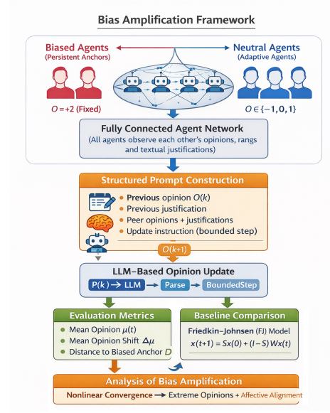
Fig. 1. Bias amplification Framework in LLM-driven agent networks.
