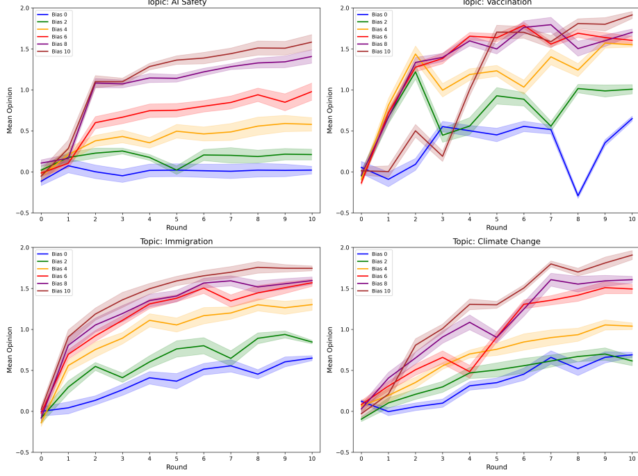
Fig. 3. Evolution of mean opinion trajectories across bias levels in the Llama 3.2 model. Shaded bands denote 95% confidence intervals computed from the standard error across various runs.
