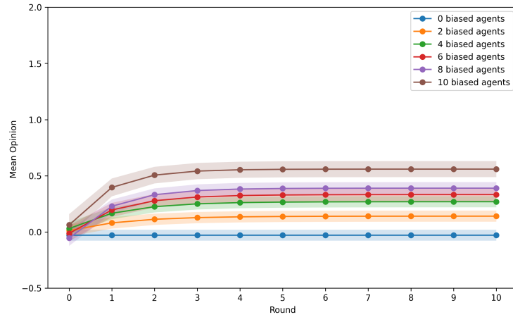
Fig. 4. Evolution of opinion distributions across bias levels for FJ Model
