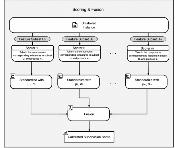
(b) Scoring and fusion. Scores from a new unlabeled instance are standardized using the normalization statistics and fused into the supervision score \kappa .
