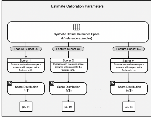
(a) Calibration. Subset-specific scorers are evaluated over the synthetic ordinal reference space to estimate normalization statistics (\mu_j, \sigma_j) .
