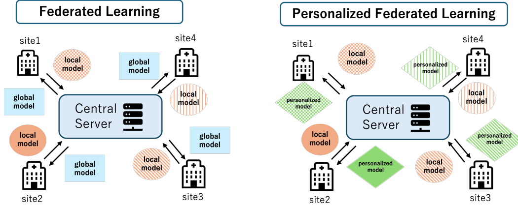
Figure 1: Images of federated learning and personalized federated learning.
