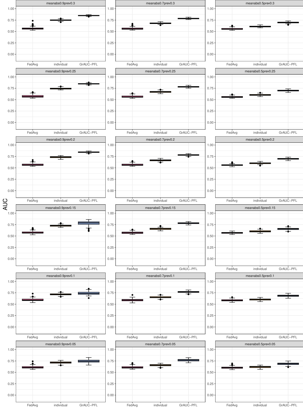
Figure 3: The results of simulation 1 in N_{z,train} = 50 . The vertical axis shows the mean AUC as assessed by the institution, whilst the horizontal axis represents the method. For each plot, 'meanabs' mentions the mean structure of \mu_{lg(z)}^* at Table 1 and 'prev' denotes the prevalence rate. The methods are as follows: 'GrAUC-PFL' refers to the proposed method, 'FedAvg' refers to the Federated Average, and 'individual' refers to the method in which models are built for each institution and their AUC are evaluated separately.
