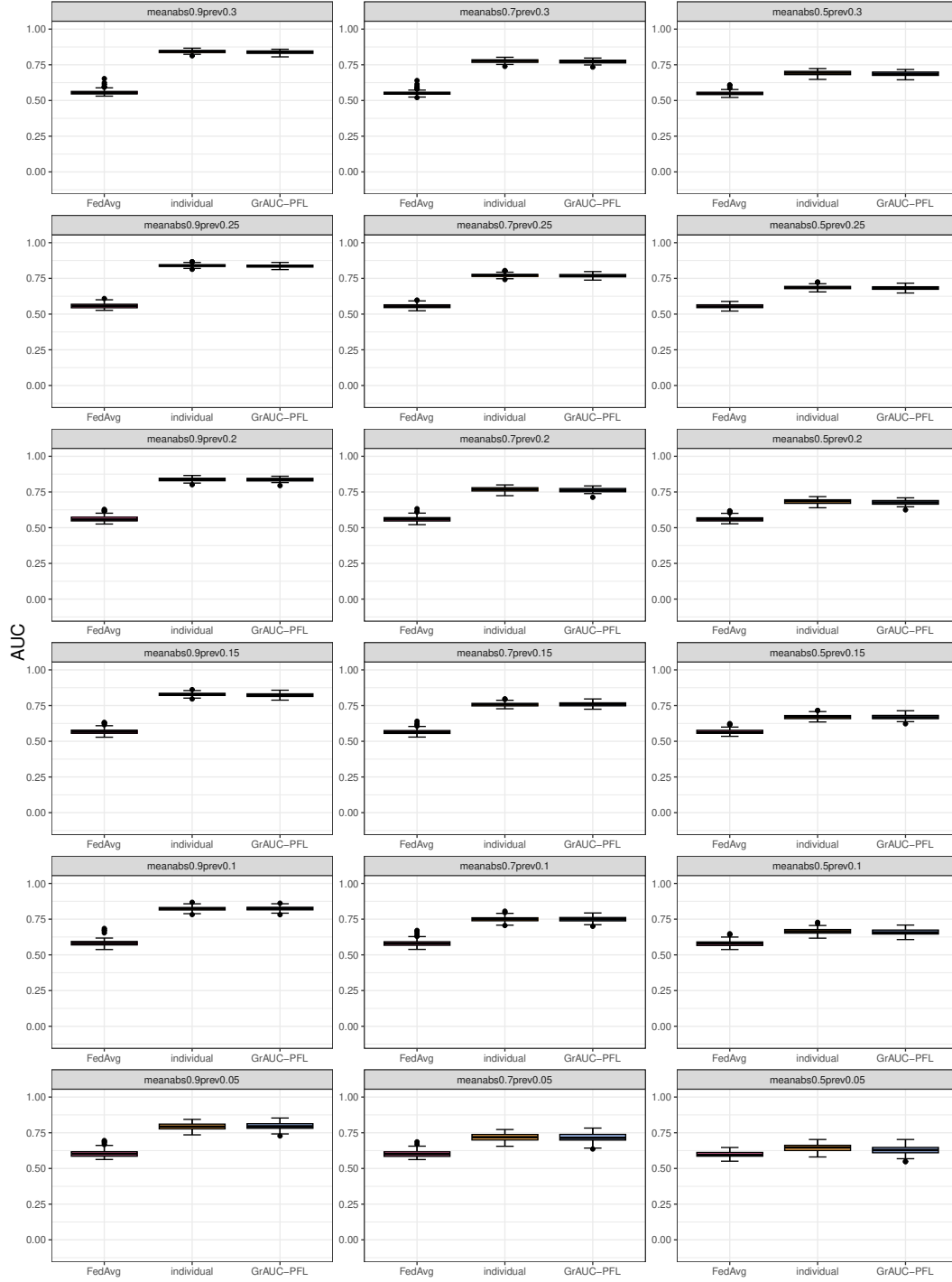
Figure 9: The results of simulation 3 in N_{z,train} = 300 .
