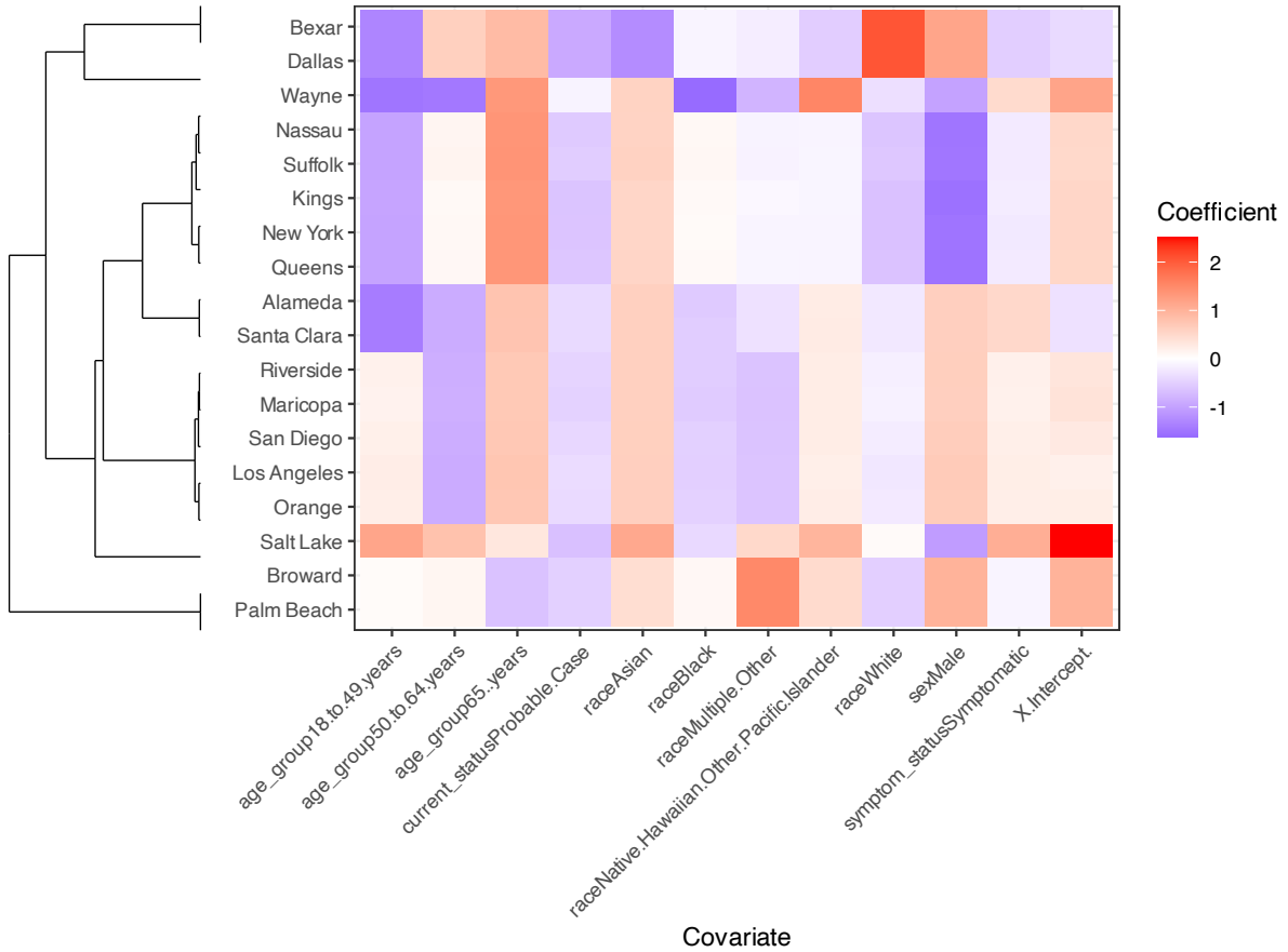
Figure 6: Heatmap of \hat{\beta} of GrAUC-PFL.
