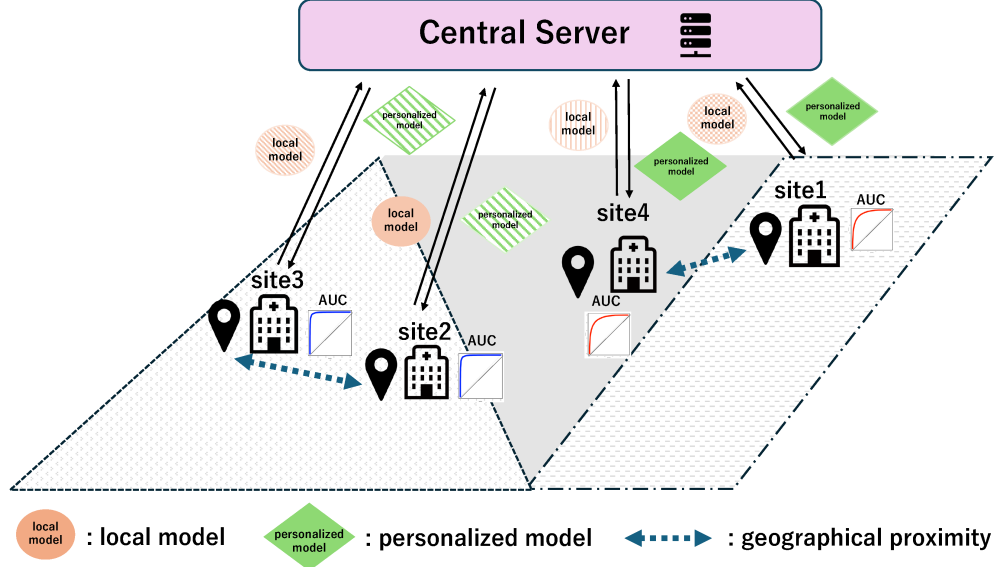
Figure 2: Image of the framework of Personalized Federated Learning considering the geographical proximity.
