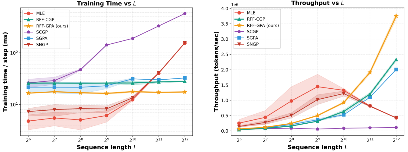
Figure 2: Training Time (Left): Training time per step as a function of sequence length L across all methods (log–log axes; shaded 95% CI). Throughput (Right): Throughput (tokens/sec) as a function of L . Curves for the inducing-point baselines (SGPA, SCGP) are continued past their largest feasible length along their fitted scaling trend.
