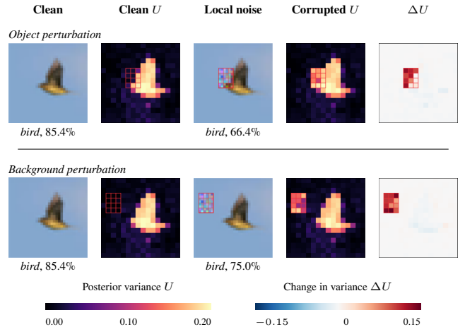
Figure 3: Localized token-wise posterior uncertainty. Object perturbation (top) and matched background perturbation (bottom). Red grids mark the 12 perturbed tokens; clean and corrupted uncertainty maps use a shared scale.
