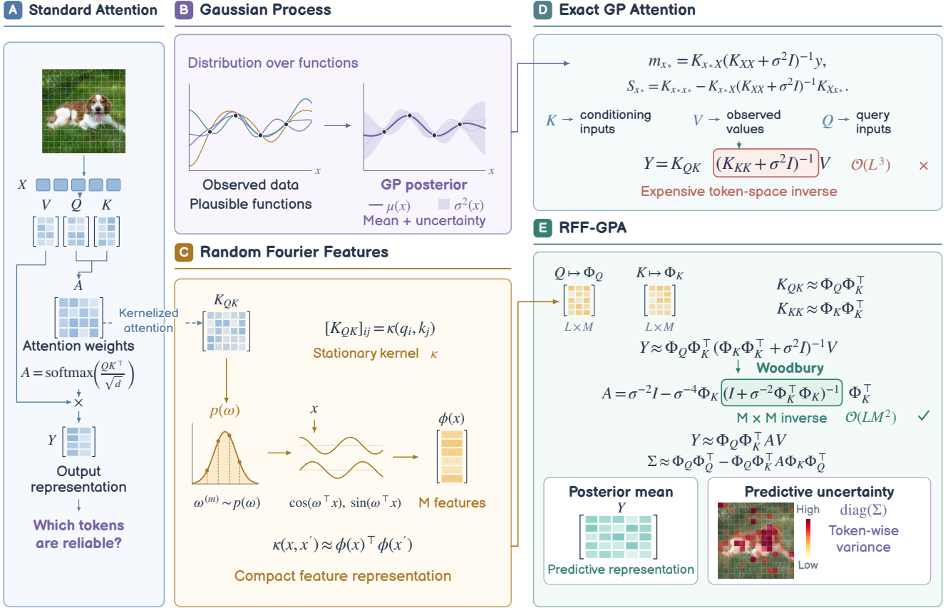
Figure 1: Overview of RFF-GPA. (A) Standard attention produces deterministic token representations without explicit uncertainty. (B,D) A GP formulation provides posterior mean and variance, but exact GP attention requires an expensive token-space inverse. (C) Random Fourier features provide a compact approximation of the stationary kernel. (E) RFF-GPA performs GP inference in the resulting feature space, replacing the L \times L inverse with an M \times M inverse while retaining the posterior mean and token-wise predictive variance.
