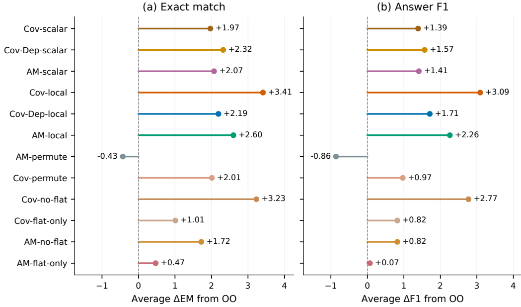
Figure 6: Differences in average EM and F1 from outcome-only training, on the same score scale as Table 1. Both scalar and local incorporation improve EM and F1 over OO for all three signals; Cov-local gives the largest gains.
