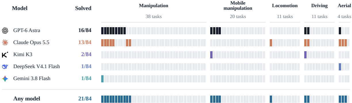
Figure 8 Success coverage across the 84 tasks. Each aligned column represents one task, grouped by its primary domain. Coloured cells indicate success and grey cells indicate failure. Tasks are ordered identically for all models, with successful tasks grouped within each domain. The bottom row marks tasks solved by at least one model: 21 tasks are covered, leaving 63 unsolved. Each model has one evaluated episode per task; counts use the outcomes at the applicable evaluation boundary.
