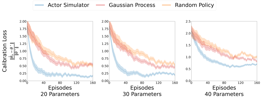
Figure 6: Comparison of calibration parameter estimation performance, i.e., \left\| \frac{\hat{\theta}_n - \theta^*}{\theta^*} \right\| , obtained by the three candidate approaches in the 20-, 30-, and 40-unknown-parameter settings. Solid curves report the mean and shaded regions denote pointwise 95% confidence intervals.
