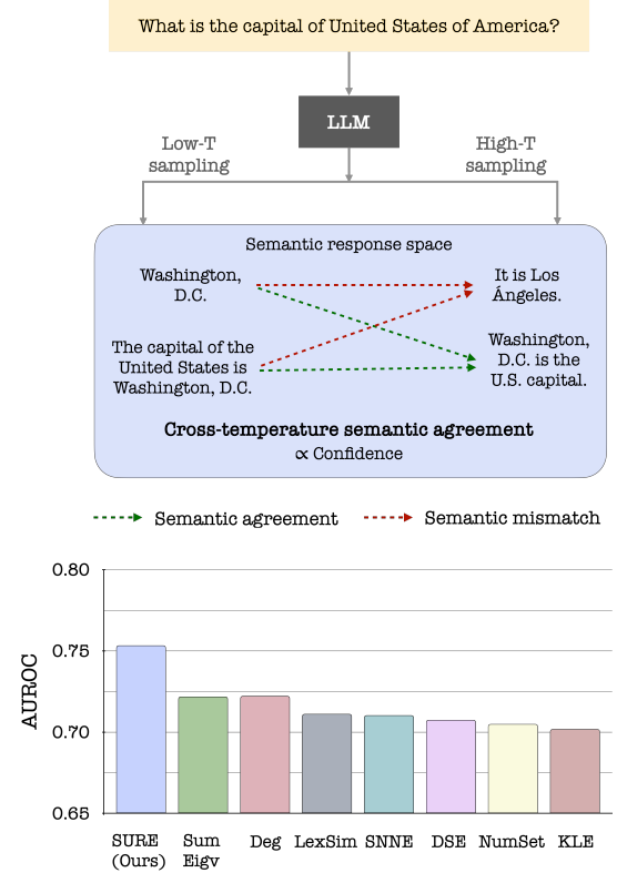
Figure 1: (Top-panel) Bipartite semantic agreement between cross-temperature responses for an example input. (Bottom-panel) SURE gives a substantial improvement in abstention AUROC over prior works on Trivia-QA. The AUROCs are averaged over 6 LLMs (Table 2).
