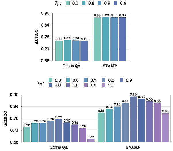
Figure 5: Temperature sensitivity of BiG-SURE. Top: Abstention AUROC when varying the anchor temperature ( T_L ), with the probe temperature fixed at ( T_H = 1.0 ). Performance remains stable across ( T_L \in \{0.1, 0.2, 0.3, 0.4\} ). Bottom: Abstention AUROC when varying ( T_H ), with ( T_L = 0.1 ). Performance generally improves as ( T_H ) approaches 0.9-1.0, while excessively high temperatures degrade performance, revealing a trade-off.
