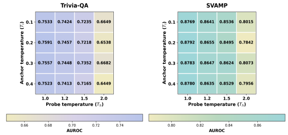
Figure 8: Temperature sensitivity analysis for SURE. Abstention AUROC for different anchor temperatures ( T_L ) and probe temperatures ( T_H ) on Trivia-QA and SVAMP. Performance is relatively stable across low-temperature anchor choices, while very high probe temperatures, especially T_H = 2.0 , reduce AUROC.
