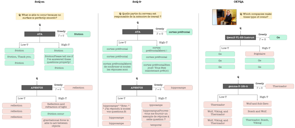
Figure 3: Illustrative examples of cross-temperature semantic agreement in multilingual and multimodal QA. For each example, we show the greedy prediction together with low-temperature anchor samples and high-temperature probe samples. Responses aligned with the ground truth are marked in green , while responses that do not align are highlighted in red . Reliable predictions exhibit strong semantic agreement across temperatures, while unreliable predictions show semantic drift and disagreement.
