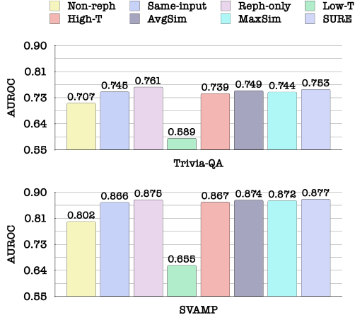
Figure 4: Ablations and direct controls for SURE. Average AUROC across the six text-QA LLMs on Trivia-QA and SVAMP for input-augmentation variants, same-temperature controls, and direct aggregation baselines. Equivalent-input augmentation and cross-temperature comparison majorly contribute to the final performance.
