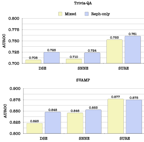
Figure 7: Effect of Rephrase-only ablation on all methods. Using Rephrase-only inputs for different methods improves them most of the time, however it comes with 2X rephrase cost.
