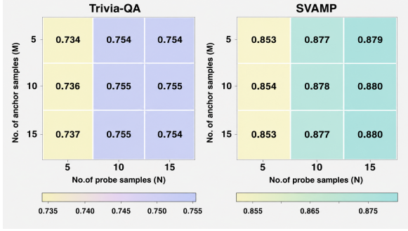
Figure 6: Sample sensitivity analysis for SURE. Abstention AUROCs averaged over LLMs for different numbers of anchor samples ( M ) and probe samples ( N ) for Trivia-QA and SVAMP.
