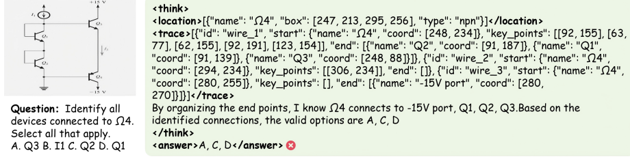
Fig. 8: Illustration of the Textual CoT reasoning process for topology analysis, detailing three sequential stages: locating, tracing, and judging.
