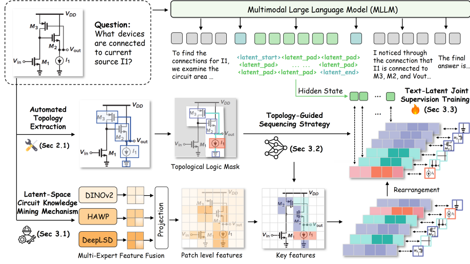
Fig. 4: Framework of Circuit-MLLM. (1) The circuit knowledge mining mechanism based on latent space provides the model with expert-level circuit representation vectors; (2) a Topology-Guided Sequencing Strategy directs latent-space reasoning to strictly follow the circuit’s topological order; and (3) Text-Latent Joint Supervision Training unifies latent-space feature alignment and explicit text supervision.
