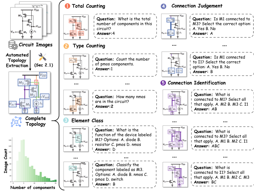
Fig. 10: Construction of Circuit-MLLM-Bench.
