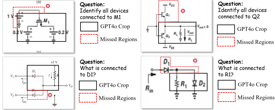
Fig. 7: Question-guided topology region cropping by GPT-4o. The black bounding boxes indicate the corresponding regions successfully cropped by the model based on the given questions, while the red dashed boxes highlight the missed regions.
