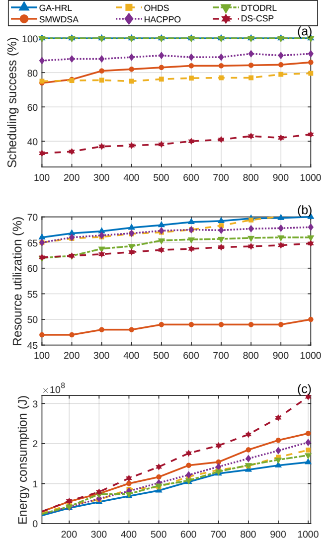
Fig. 6: Effect of the number of workflows K with \lambda = 0.5 , v = 0.1 , and \alpha^{df} = 2.1 : (a) workflow scheduling success rate, (b) average container resource utilization, and (c) total system energy consumption.
