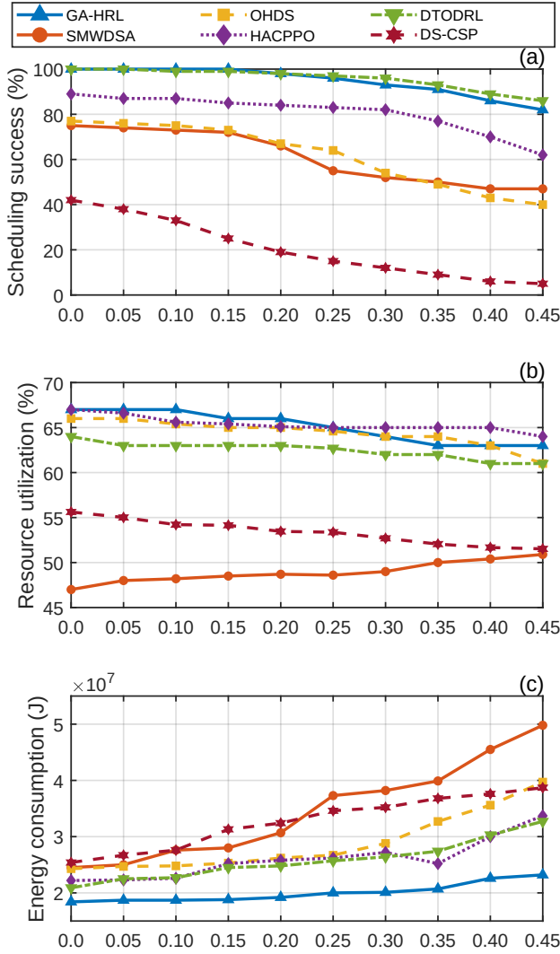
Fig. 5: Effect of the execution-speed variation coefficient v with K = 100 workflows, \lambda = 0.5 , and \alpha^{df} = 2.1 : (a) workflow scheduling success rate, (b) average container resource utilization, and (c) total system energy consumption.
