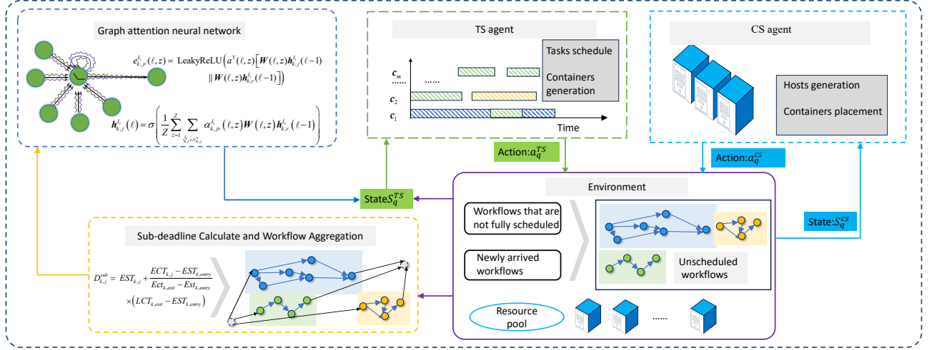
Fig. 2: Schematic diagram of the GA-HRL scheduling algorithm.
