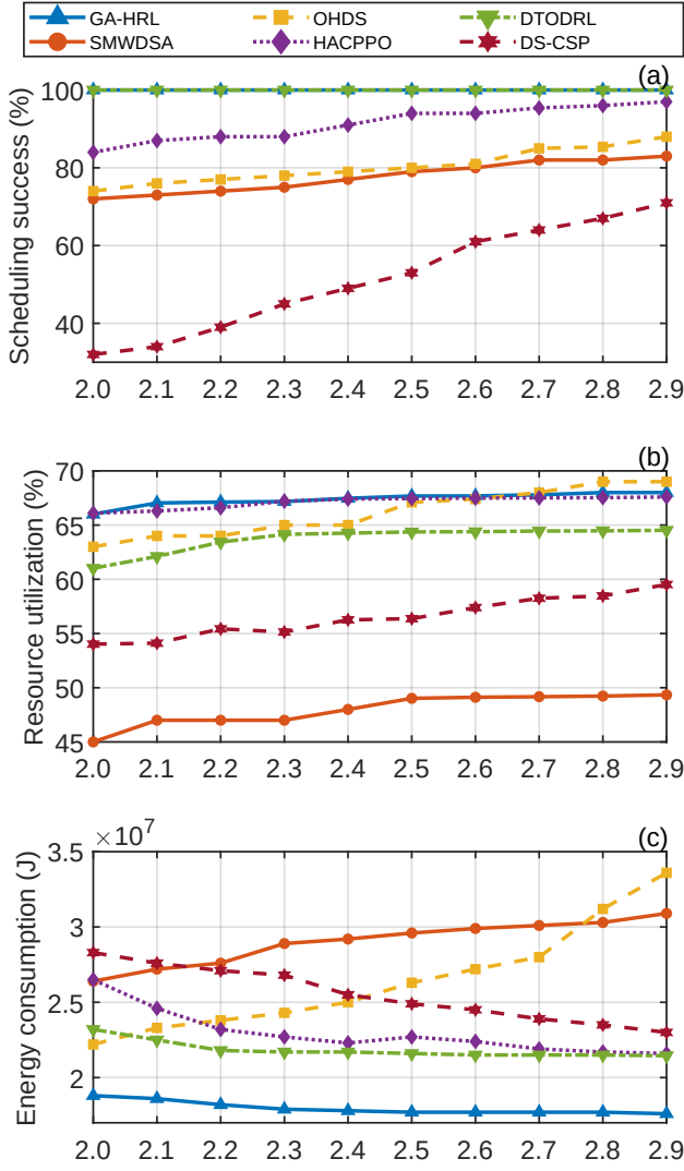
Fig. 4: Effect of the deadline factor \alpha^{df} with K = 100 workflows, \lambda = 0.5 , and v = 0.1 : (a) workflow scheduling success rate, (b) average container resource utilization, and (c) total system energy consumption.
