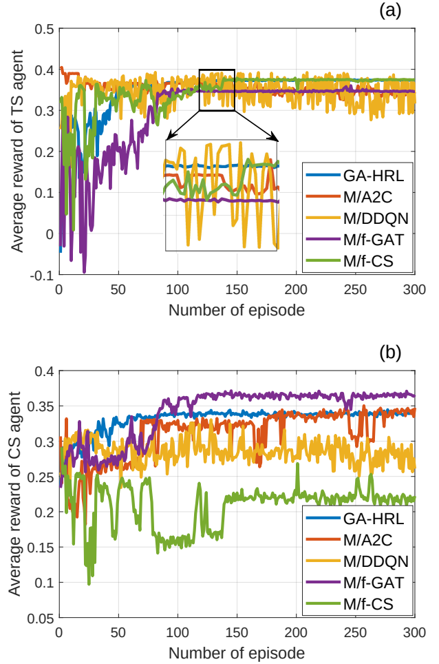
Fig. 3: Training convergence of different methods: (a) average reward of the TS agent and (b) average reward of the CS agent.
