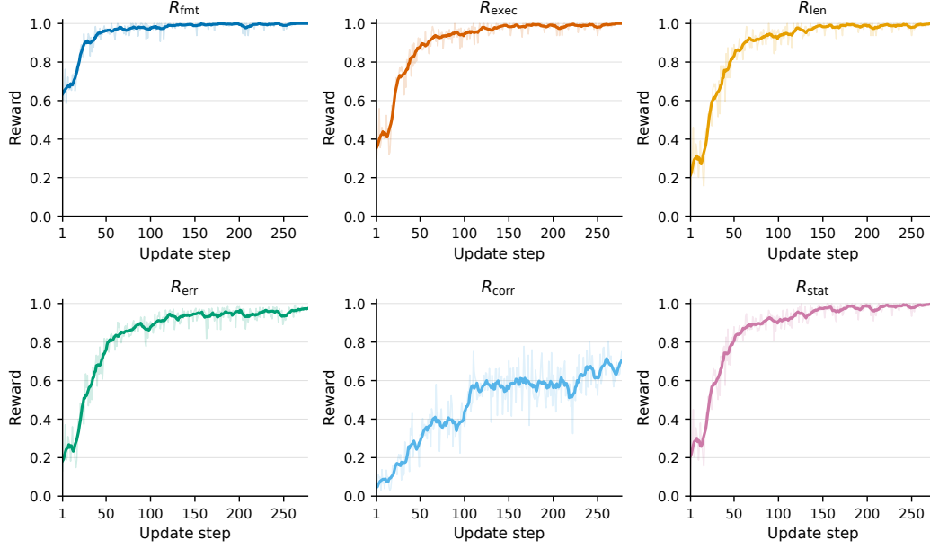
Figure 8: Training dynamics of the six RLVR reward functions.
