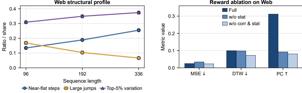
Figure 7: Web benchmark analysis. Left: target-window statistics for Web, where near-flat steps are normalized adjacent differences no larger than 0.01, large jumps are differences at least 0.20, and top-5% variation is the share of total variation contributed by the largest 5% adjacent changes. Right: reward ablation on Web averaged over lengths 96, 192, and 336. Removing correlation and statistic rewards can reduce MSE and DTW while sharply reducing Pearson correlation, showing that low pointwise or warped error does not necessarily imply event-shape preservation on Web.
