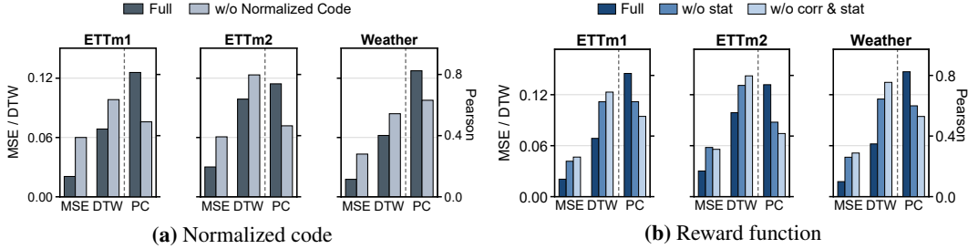
Figure 4: Ablation results for normalized code representation and reward design. Panel (a) studies normalized code, and panel (b) studies reward components.
