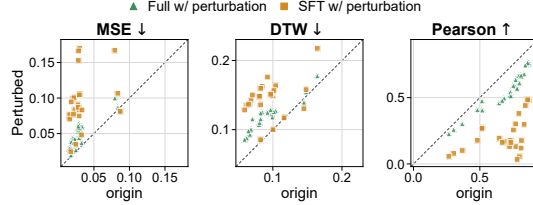
Figure 5: Template robustness analysis under perturbed descriptions.
