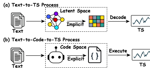
Figure 1: Illustration of the Text-to-TS process and the proposed Text-to-Code-to-TS process.
