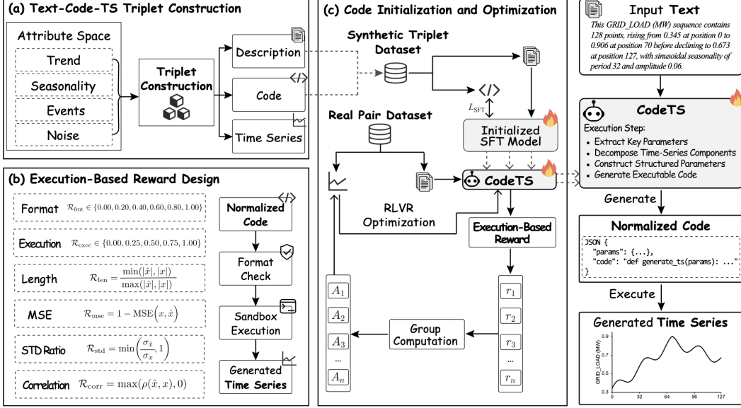
Figure 2: Overview of CodeTS. (a) Synthetic Text-Code-TS triplets are constructed from structured temporal attributes. (b) Execution-based rewards verify normalized format, code executability, and time series quality. (c) The model is first initialized on synthetic triplets by SFT and then optimized on real Text-TS pairs with execution-based rewards and GRPO. At inference time, CodeTS maps input text to normalized code and executes it to generate the target time series.
