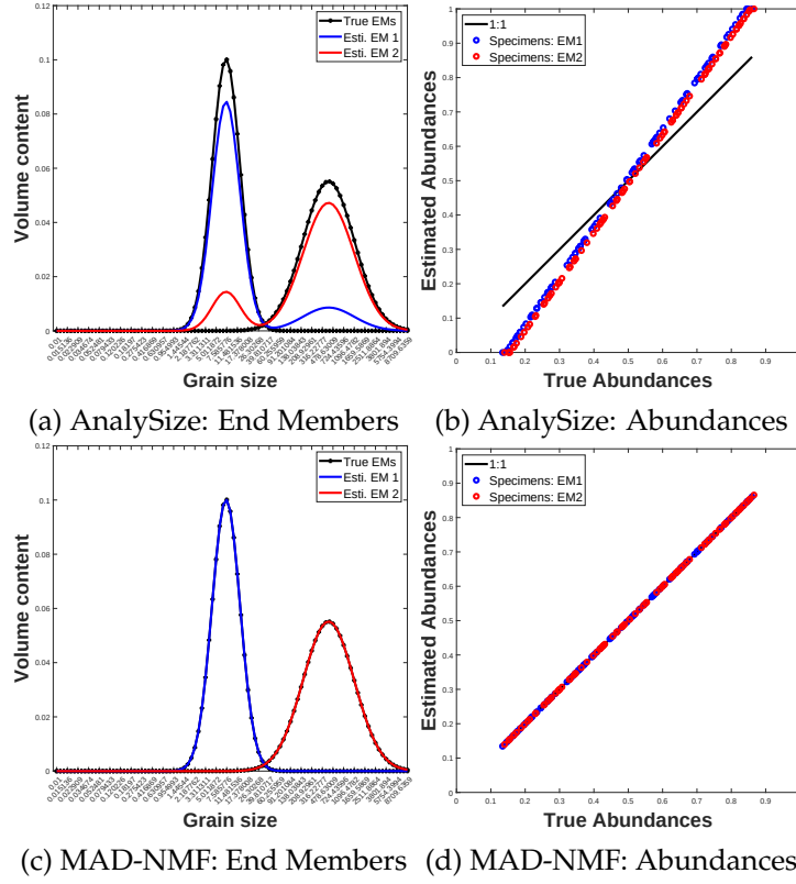
Figure 2: Highly mixed two-end-member dataset: \alpha = 5 , \lambda = 1 (a and b) AnalySize; (c and d) MAD-NMF.
