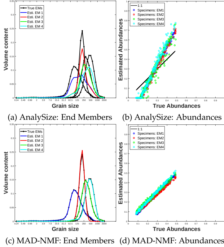
Figure 5: Noisy highly mixed coversand dataset: \alpha = 100 , \lambda = 3.3 (a and b) AnalySize; (c and d) MAD-NMF.
