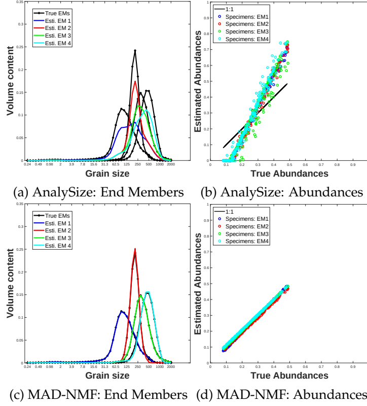
Figure 4: Highly mixed coversand dataset: \alpha = 100 , \lambda = 3.5 (a and b) AnalySize; (c and d) MAD-NMF.
