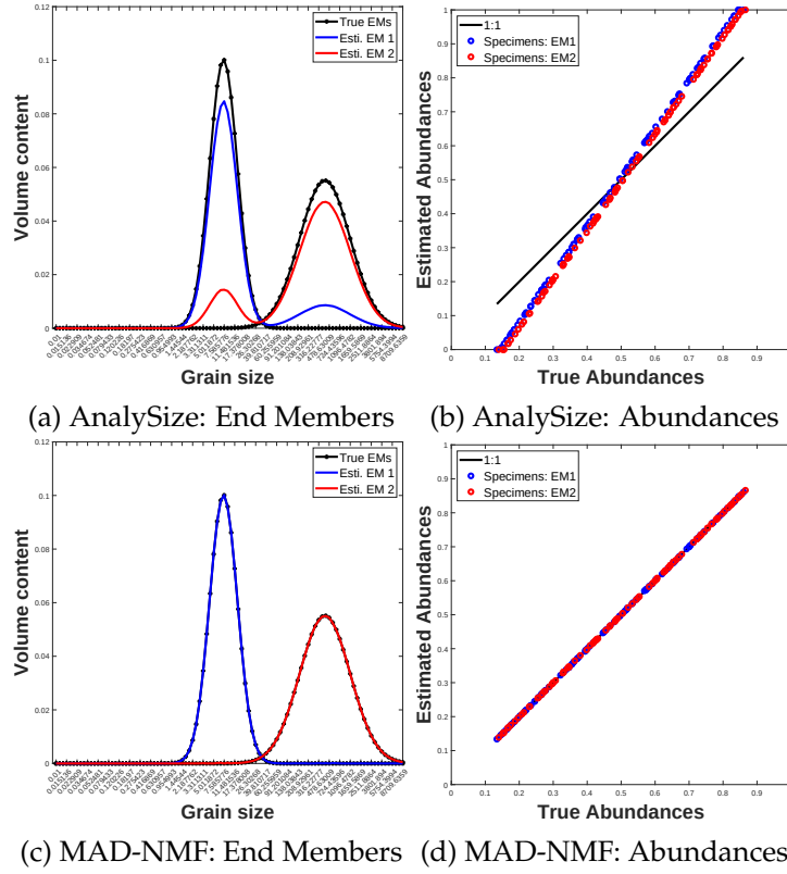
Figure 3: Noisy highly mixed two-end-member dataset: \alpha = 5 , \lambda = 1 (a and b) AnalySize; (c and d) MAD-NMF.
