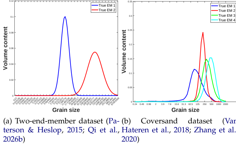
Figure 1: True end members
