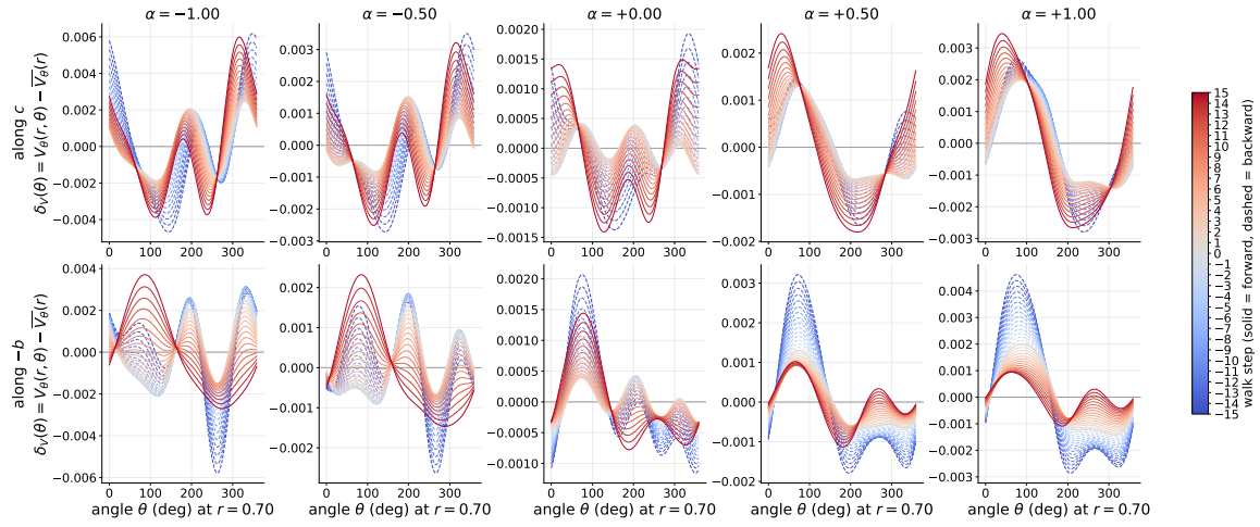
Figure 4: Angular deviation profiles for the ASRNN trained to model the Mexican hat potential for various values of \alpha unseen during training. Top: symmetry-directed flow along c^* . Bottom: equivariance-directed flow along b^* . Here the direction is computed once at t = 0 and kept fixed, i.e. the FIXED trajectory.
