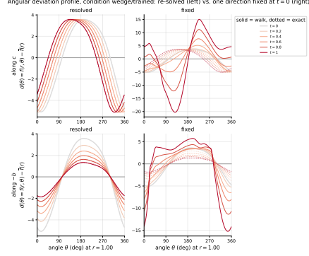
Figure 7: Angular deviation profiles for the wedge-trained classifier. Top: symmetry-directed flow along c^* ; bottom: equivariance-directed flow along b^* . Left: the local direction is recomputed at every step; right: the initial direction is kept fixed. Solid curves denote the realised trajectory, dotted curves the ideal function-space evolution.
