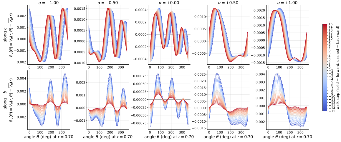
Figure 3: Angular deviation profiles for the ASRNN trained to model the Mexican hat potential for various values of \alpha unseen during training. Top: symmetry-directed flow along c^* . Bottom: equivariance-directed flow along b^* . Here the local direction is recomputed at every step, i.e. the RESOLVED trajectory.
