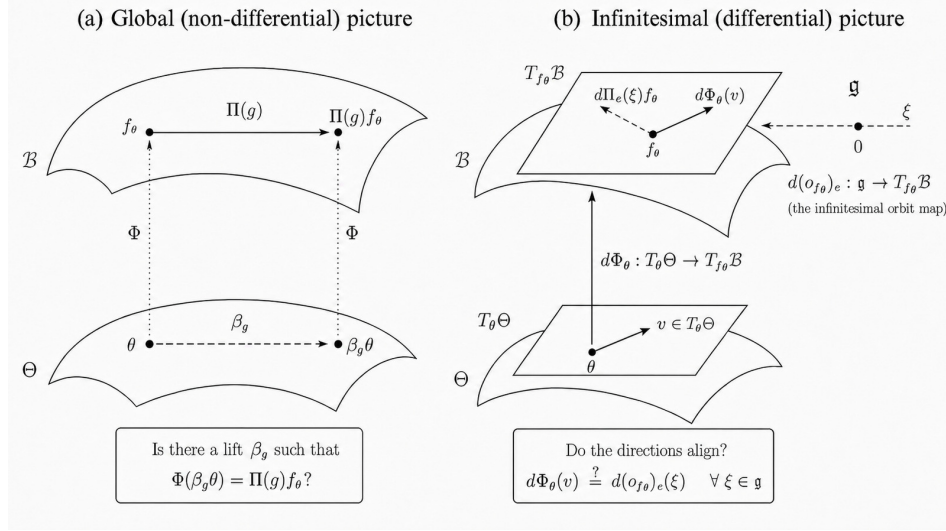
Figure 2: Global and infinitesimal lifting through the neural-network realisation map. Left: can a symmetry transformation in function space be realised by a transformation in parameter space? Right: do the infinitesimal symmetry directions lie in the function-space tangent directions accessible through the parametrisation?
