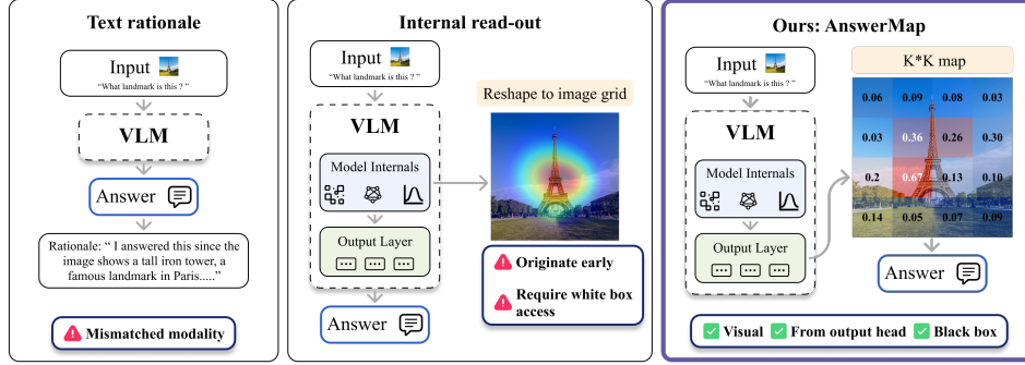
Figure 1: Three ways to explain one frozen VLM’s answer. A text rationale is in a mismatched modality. An internal read-out is in the right modality but originates too early and needs the weights. AnswerMap reads the output head one band at a time, the map is visual and black-box, and a fixed read-out computes the answer from it.
