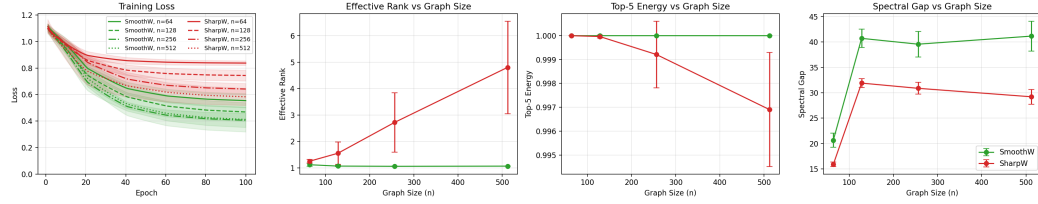
Figure 3: Training dynamics and spectral summaries under synthetic graphon families. Left: training loss for SmoothW and SharpW at increasing sizes. Middle/right: spectral summaries of the estimated attention graphons (effective rank, top-5 energy, and spectral gap) as size grows. Metrics are defined in Appx F.2.
