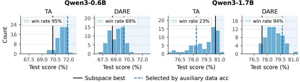
Figure 5: S-RandOpt sampled weights' test performance. We sample 64 random weights in language models using S-RandOpt, and compare their test performance with the best point on the task-vector subspace (subspace best). A high proportion of sampled weights from outside the subspace outperforms the best weight on the subspace (Subspace best).
