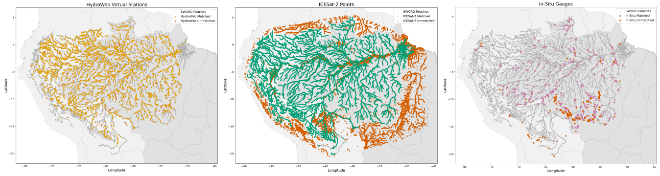
Figure 14: Spatial distribution of data sources in AmazonWSE, matched (kept) and unmatched (discarded) to SWORD reaches within 10 km ( before quality filtering). From left to right: HydroWeb virtual stations, ICESat-2 transects, and ANA in situ gauges.
