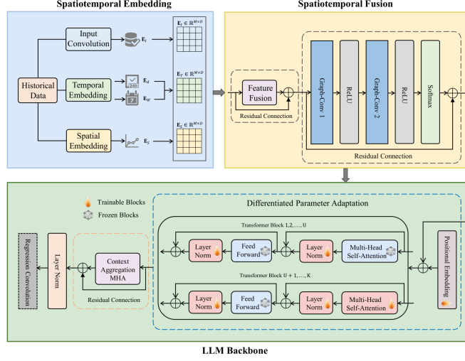
Fig. 1. The framework of DF-LLM.
