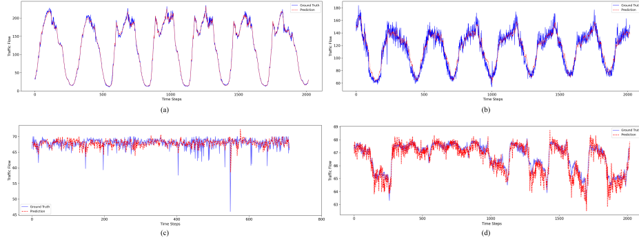
Fig. 2. Comparison of DF-LLM predictions with ground-truth values on four datasets: (a) PEMS04; (b) PEMS08; (c) METR-LA; (d) PEMS-BAY.
