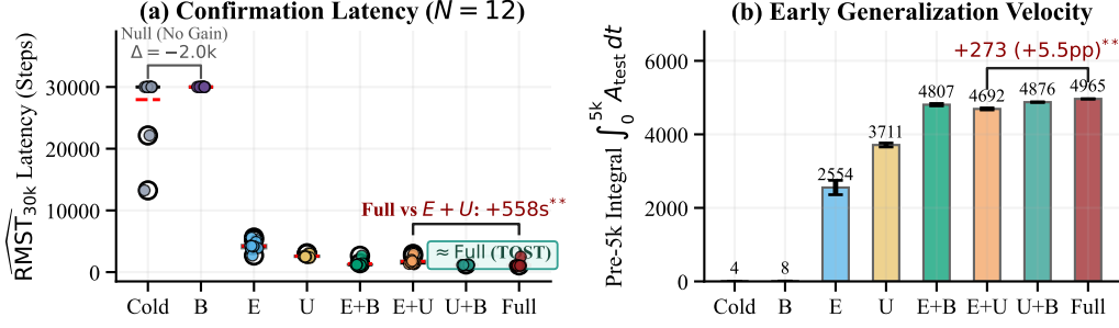
Figure 2: Component Localization and Factorial Synergy ( N = 12 Formal Blocks 210–221: 96 Factorial Runs plus 12 Scale Controls, 108 Runs Total). (a) Confirmation latency \text{RMST}_{30k} across 8 factorial conditions (medians and individual points). Full transfer accelerates confirmation by +558.3 steps over representation transfer E + U (Holm p = 0.0088 ). Crucially, co-transferring readout and internal blocks ( U + B ) achieves TOST equivalence to full transfer ( p = 0.0011 , \Delta = -16.7 steps), while internal blocks alone ( B ) do not establish a confirmation benefit within the 30k horizon ( p = 0.50 ). (b) Pre-5k accuracy integral, confirming that full transfer provides +5.46 pp higher early accuracy than E + U (Holm p = 0.0039 ).
