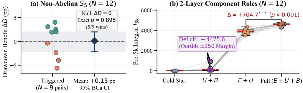
Figure 3: Generality and Dynamical Boundaries. (a) Non-abelian S_5 dynamic protection ( N = 12 prospective blocks, 9 triggered pairs): carrier shielding shows no confirmed drawdown benefit ( \Delta D = +0.15 \pm 1.14 pp, exact p = 0.895 ). (b) Two-layer component roles ( I_{5k} , N = 12 fresh blocks): internal blocks accelerate acquisition (+704.67 units, p < 0.001 ), while omitting donor embeddings ( U + B ) incurs a -4475.63 -unit deficit exceeding the pre-specified \pm 250 -unit equivalence margin.
