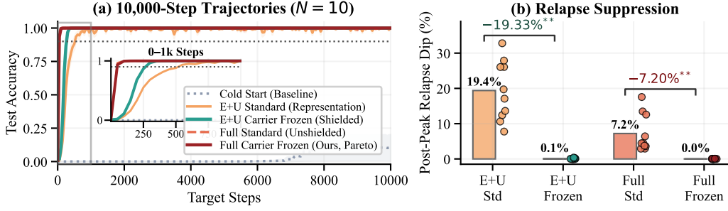
Figure 1: Separating takeoff velocity from trajectory stability ( N = 10 Blocks 230–239: 60-run confirmatory matrix plus 10-run exploratory extension). (a) Test-accuracy trajectories ( \pm SEM). Full transfer reaches 90% by step 50, versus 250–500 steps for representation conditions. (b) Freezing E + U reduces post-peak relapse from 19.40% to 0.07% (Holm p = 0.005859 ). The exploratory full_carrier_frozen extension combines 50-step takeoff with 0.02% relapse.
