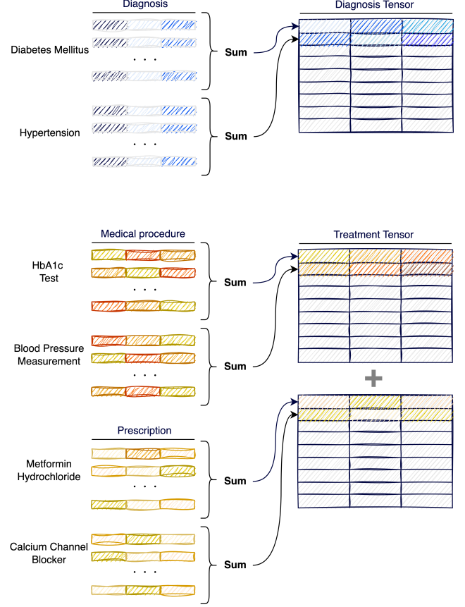
Figure A.4: Flow diagram illustrating the embedding block. During the diagnostic process, sub-tokens are initially transformed into vectors, which are then aggregated to generate a singular “diagnosis” vector. Similarly, sub-tokens related to medical procedures and prescriptions undergo embedding into vectors and, following aggregation, form “medical procedure” and “prescription” vectors, respectively. These two vectors are subsequently concatenated to represent treatment information. It is essential to note that when dealing with a month’s worth of medical claims data, encompassing numerous diagnoses, medical procedures, and prescriptions, both diagnostic and treatment information is presented as tensors. These tensors possess dimensions of batch size, length, embedding size, with the length typically spanning several dozen.
