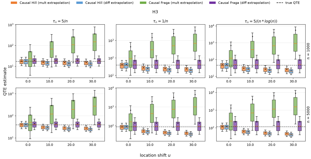
Figure 4: Quantile treatment effect estimations under the location shift u for model H_3 . The boxplot whiskers correspond to the 0.1 and 0.9 quantiles, the orange line is the median, and the black dots are the means.
