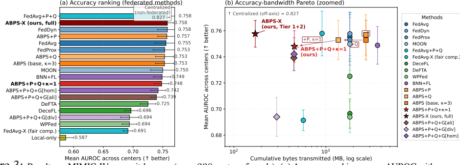
Figure 3: Results on MIMIC-IV careunit-by-year ( n = 230 centers, 5 seeds). (a) Accuracy ranking: mean AUROC with across-seed std, color-coded by method family (blue: star-topology FL, green: decentralized, orange: ABPS+P/Q, red: ABPS-X, purple/brown: goal-aware, olive: local-only). The dashed line denotes the non-federated centralized upper bound (off-axis). (b) Accuracy vs. bandwidth Pareto (log-scale bandwidth): ABPS-X (dark-red star) matches FedDyn’s AUROC (0.758) at 0.09\times FedAvg bandwidth. Red arrows show the ablation path \text{ABPS} \rightarrow \text{P} \rightarrow \text{Q} \rightarrow \text{P+Q+}\kappa=1 \rightarrow \text{ABPS-X} , with each step improving the trade-off. 0.50\times , a modest improvement, but cannot reach \kappa=1 because the star topology has no mechanism for selecting a single best peer. The full ABPS-X variant adds 2-layer personalization, server-side EMA momentum \beta=0.5 , 15-dim goal-aware metadata under the homogeneity goal, and validation-AUROC early stopping (patience 10 of 100), reaching 0.758 \pm 0.010 at 0.09\times FedAvg with tighter variance than FedDyn. The same-extension FedAvg-X fair comparator drops to 0.691 \pm 0.008 , 6.7 AUROC points behind ABPS-X: 2-layer personalization over-adapts each private head when the star topology averages across all 230 peers, whereas ABPS’s \kappa=1 Bayesian selection supplies the one-peer constraint under which personalization helps. Empirical isolation does not activate here ( \mathbb{E}[|\mathcal{P}_i|] \approx 1.00 when \kappa=1 ), but the goal-aware filter of the next subsection engages Lemma 1’s rest regime in up to 41% of rounds.
