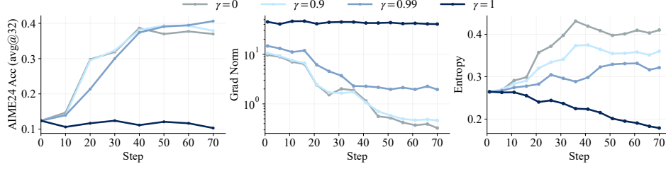
Figure 4: Training dynamics under different \gamma . OPD distills a Qwen3-4B-Math teacher into a Qwen3-1.7B student, with validation accuracy, gradient norm, and policy entropy reported.
