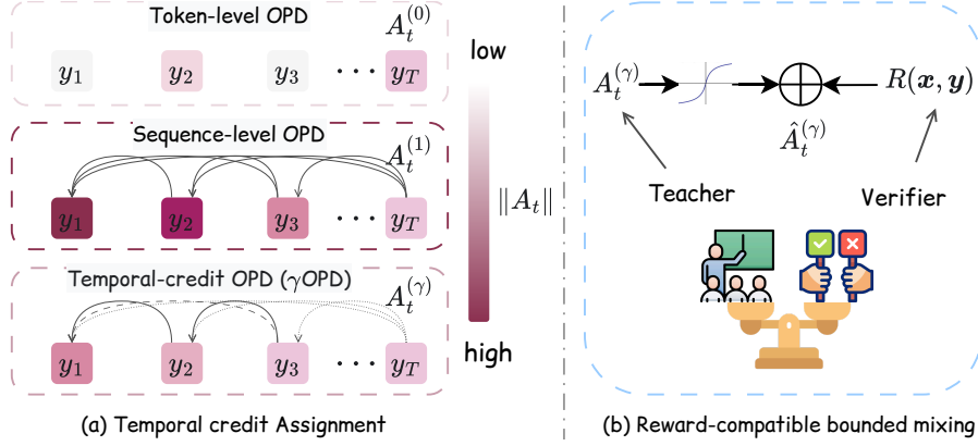
Figure 2: Overview of \gamma OPD. (a) Token-level OPD considers only the log-ratio of the current token, whereas sequence-level OPD accumulates the log-ratios of all future tokens. \gamma OPD introduces a discount factor \gamma to interpolate between these two extremes. (b) The \gamma OPD advantage is first normalized and then combined with the verifiable task reward, balancing dense teacher guidance with task-level verification signals.
