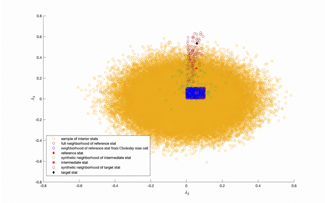
Figure 7: Synthetic neighborhoods of the target and intermediate statistics fixed in Fig. 6 for G_3 .
