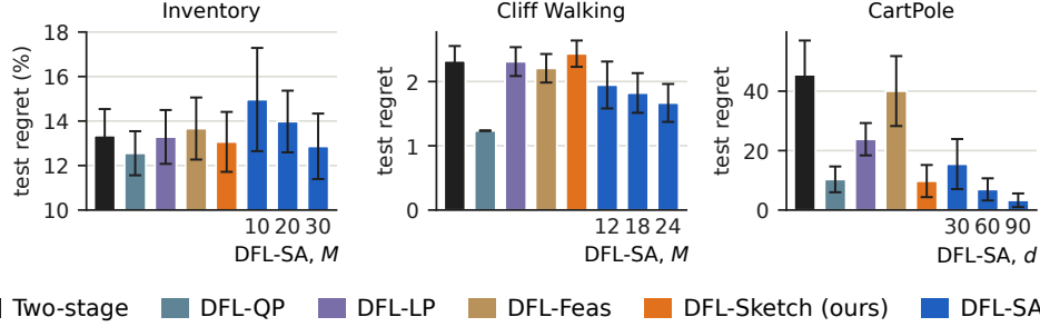
Figure 3: Test regret on three tasks (lower is better). DFL-Sketch improves over DFL-LP on Inventory and CartPole, showing the benefit of smoothing across basis changes. DFL-SA further achieves regret close to DFL-QP at substantially lower cost.
