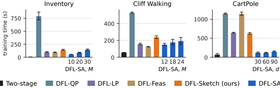
Figure 4: Total training time for different tasks. DFL-QP is the most expensive method because it differentiates through the full KKT system. DFL-Sketch adds overhead from solving multiple sketched LPs, while DFL-SA reduces this cost through state aggregation.
