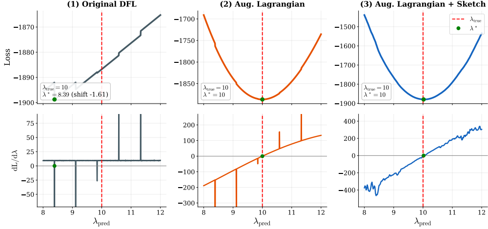
Figure 1: Loss (top) and gradient (bottom) of three DFL objectives as \lambda_{\text{pred}} varies; red dashed indicate \lambda_{\text{true}} and green dots indicate the loss minimum. (1) The occupancy proxy has a shifted minimum. (2) The augmented Lagrangian has a minimum at the true parameter. (3) Sketch averaging empirically reduces boundary sensitivity.
