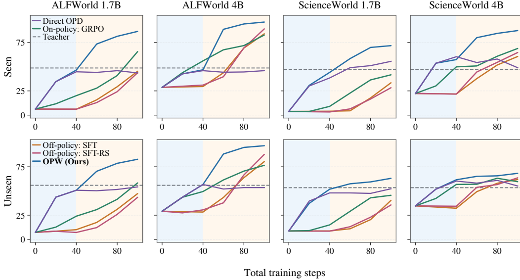
Figure 2: Task performance during warmup and GRPO.
