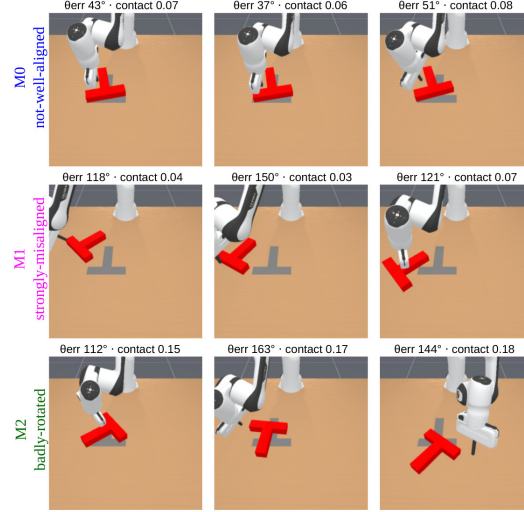
Figure 5: Failure modes discovered on Push-T (image). Each row shows 3 members of a single geometric cluster. Labels are assigned by the naming pipeline from the task-store vocabulary.
