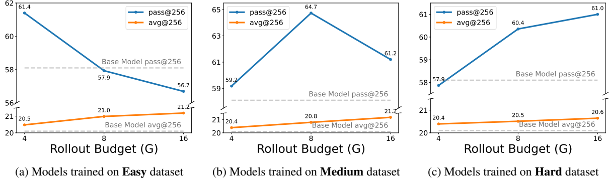
Figure 1: \text{avg}@256 and \text{pass}@256 performance across different rollout budgets for models trained on different difficulty subsets.
