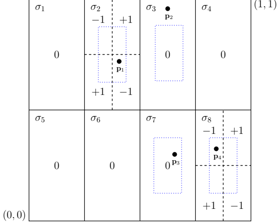
(a) Illustration of a value function g_{\mathbf{k}} in the 2D grid \mathcal{G}_{\mathbf{k}} with \mathbf{k} = (2, 1) . There are 4 points \mathbf{p}_1, \mathbf{p}_2, \mathbf{p}_3, \mathbf{p}_4 with w_{\mathbf{p}_1}, w_{\mathbf{p}_2}, w_{\mathbf{p}_4} > 0 and w_{\mathbf{p}_3} < 0 . The blue boxes show the center sub-cells. \sigma_2, \sigma_8 are positively good cells, and are split into four sub-cells to assign different values.
