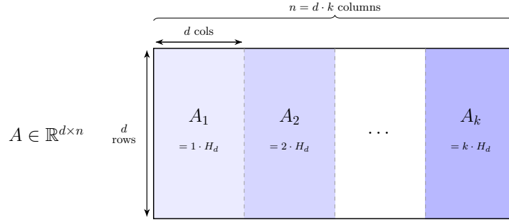
Figure 2: Illustration of the block construction. Each submatrix A_i is a i -scaled copy of a Hadamard matrix, and corresponds to the subsequence P_i .
