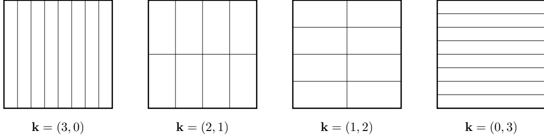
Figure 3: Illustration of different grid constructions when d = 2 and m = 8 .
