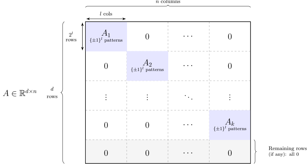
Figure 1: Illustration of the block construction. Each submatrix A_i corresponds to a subsequence P_i , and the rows of A_i are distinct \{\pm 1\} -patterns of length l .
