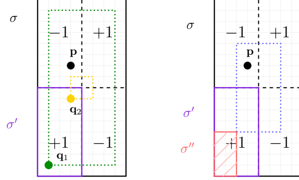
Figure 5: Illustration of the contribution from the grid points inside a positively good cell \sigma to \sum_{\mathbf{q}: \mathbf{q} \geq \mathbf{p}} g_{\mathbf{k}, \mathbf{q}} for a point \mathbf{p} contained in \sigma . In the left figure, the green (yellow) box represents the box formed by \mathbf{q}_1 ( \mathbf{q}_2 ) and its reflections. The contribution from the 4 grid points which form the green (yellow) boxes is 1 (0). In the right figure, the blue box represents the center sub-cell of \sigma . For every grid point in the red box, the contribution from it and its reflections is 1.
