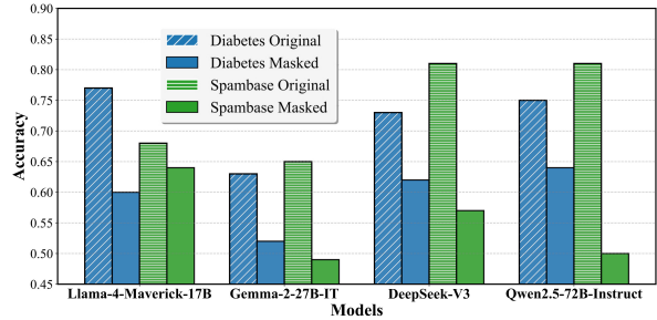
Figure 1: The test accuracy of LLMs with or without the metadata about the dataset.
