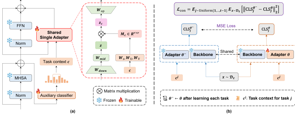
Figure 2: Illustration of FACET. (a) Task-conditioned feature transformation within a single adapter. We predict the task context c and use it to generate a transformation matrix M_c to obtain task-dependent features. Activation functions are not shown for simplicity. (b) Task-conditioned feature consistency objective when training on a new task t with dataset \mathcal{D}_t .
