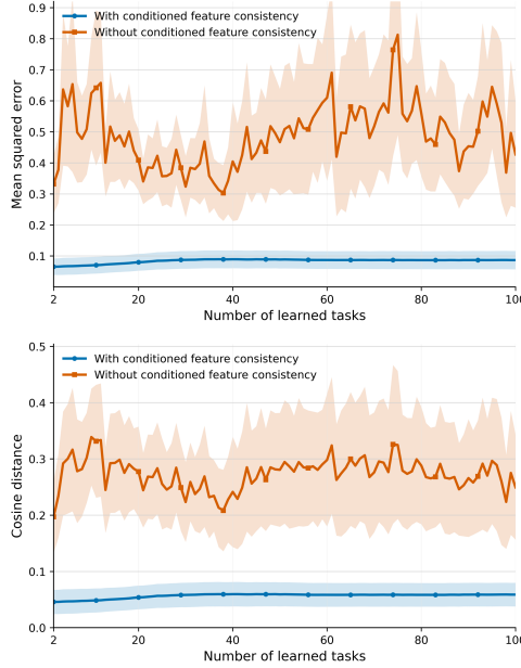
Figure 3: How well our single adapter preserves the feature distribution of the first task as it is sequentially trained on new tasks from task 2 to 100. Top: Mean square error as the distance metric. Bottom: Cosine distance as the distance metric. We compute the distance between the CLS feature produced by the model after it has learned the first task with the corresponding CLS feature after the model has sequentially learned t \in \{2, \dots, 100\} tasks. The original training data and context for the first task are used for a direct comparison.
