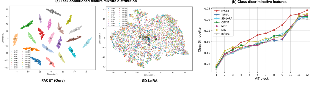
Figure 1: Comparison of feature distributions. (a) t-SNE of block 1 features, colored based on task . FACET shows well-separated task-specific distributions, while SD-LoRA’s are mixed. (b) Class -averaged silhouette score (higher values mean better intra-class compactness and inter-class separation) across blocks. FACET achieves higher scores than representative LoRA-based (SD-LoRA) and per-task adapter based (TUNA) methods, producing more class-discriminative features that are beneficial for classification.
