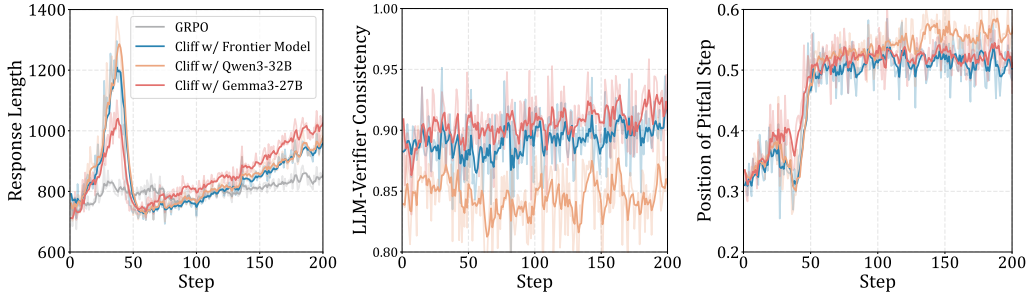
Figure 2: Training plots of GRPO and Cliff with different teachers 6 . The student model is Phi-4-Mini-Instruct trained on the math domain.
