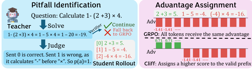
Figure 1: Overview of Cliff .
