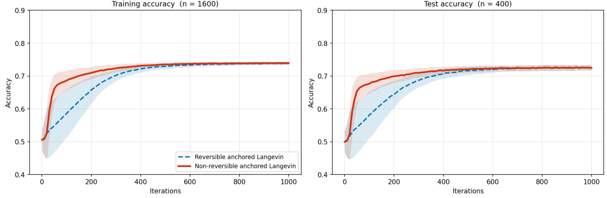
Figure 5: Accuracy over the training set and the test set for the synthetic data. The red part (solid line) denotes the mean and standard deviation of the non-reversible anchored Langevin algorithm with J_s(x) ( \alpha = 1 ) and the blue part (dashed line) denotes the mean and standard deviation of the reversible anchored Langevin algorithm ( \alpha = 0 ).
