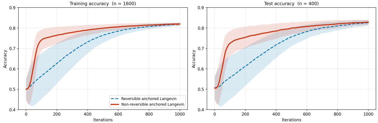
Figure 6: Accuracy over the training set and the test set for the synthetic data. The red part (solid line) denotes the mean and standard deviation of the non-reversible anchored Langevin algorithm with J_g(x) ( \alpha = 1 ) and the blue part (dashed line) denotes the mean and standard deviation of the reversible anchored Langevin algorithm ( \alpha = 0 ).
