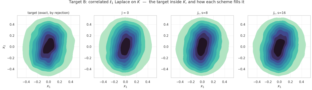
Figure 4: Visualized density plots of the first two coordinates (x_1, x_2) for target (B), U(x) = \|L^{-1}x\|_1 in (7.15), restricted to the ball K in (7.16). From left to right: 5000 exact samples of the target obtained by rejection, and the walkers of the reversible projected anchored Langevin algorithm ( J = 0 ) and of NRALD with J_s in (2.26) for s = 8 and s = 16 after 5000 iterates with \eta = 5 \times 10^{-4} (8 replicas of 5000 walkers), shown as kernel density estimates with the same contour levels.
