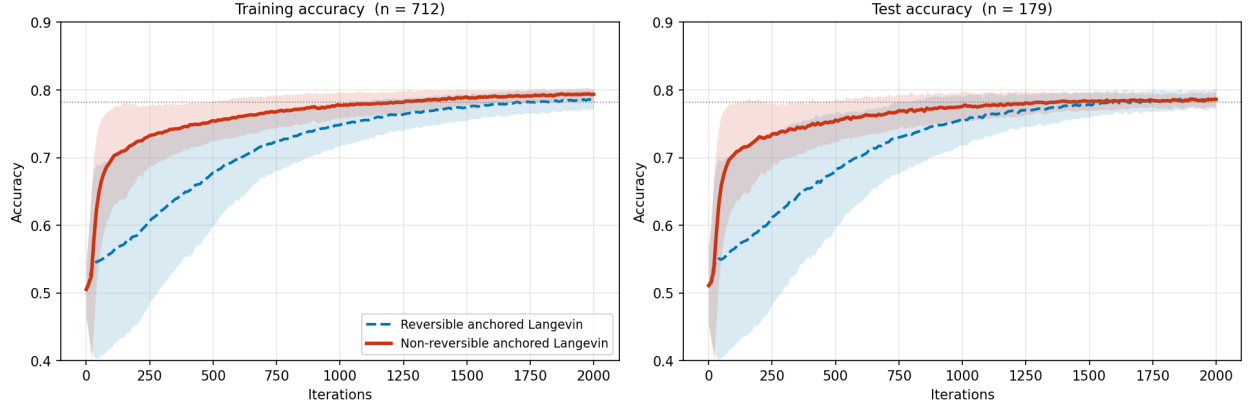
Figure 9: Accuracy over the training set and the test set for the Titanic dataset over the unit ball. The red part (solid line) denotes the mean and standard deviation of the non-reversible anchored Langevin algorithm with J_s(x) ( \alpha = 1 ), the blue part (dashed line) denotes the mean and standard deviation of the reversible anchored Langevin algorithm ( \alpha = 0 ), and the grey dotted line is the test accuracy of the Bayesian logistic regression fit.
