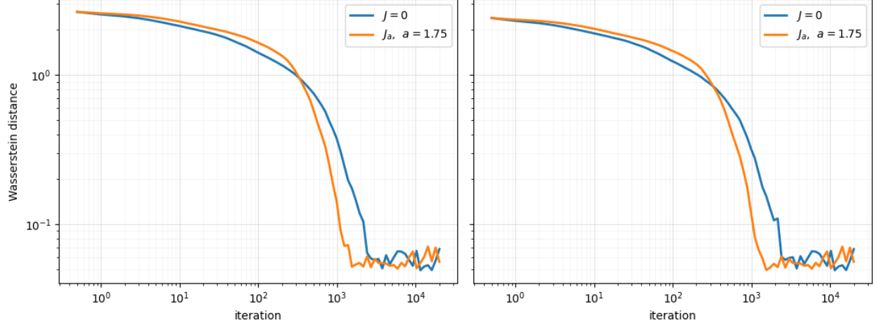
Figure 1: 2-Wasserstein distance between the particle distribution and an exact sample of the target (7.5) with the MCP regularizer (7.6), as a function of the iterate on logarithmic axes, for the reversible anchored Langevin algorithm ( \alpha = 0 ) and NRALD with the constant skew-symmetric matrix J_a ( \alpha = 1 , a = 1.75 ), averaged over 5 replications of N = 5000 particles, from the initial distributions \mathcal{N}(0, 10 I_d) (left) and \mathcal{U}(-5, 5)^d (right).
