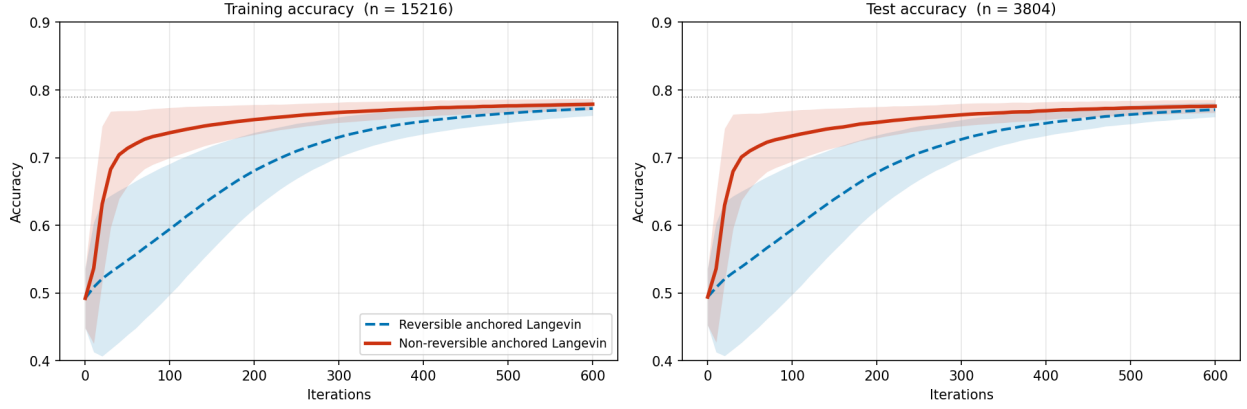
Figure 7: Accuracy over the training set and the test set for the Telescope dataset over the unit ball. The red part (solid line) denotes the mean and standard deviation of the non-reversible anchored Langevin algorithm with J_s(x) ( \alpha = 1 ), the blue part (dashed line) denotes the mean and standard deviation of the reversible anchored Langevin algorithm ( \alpha = 0 ), and the grey dotted line is the test accuracy of the Bayesian logistic regression fit.
