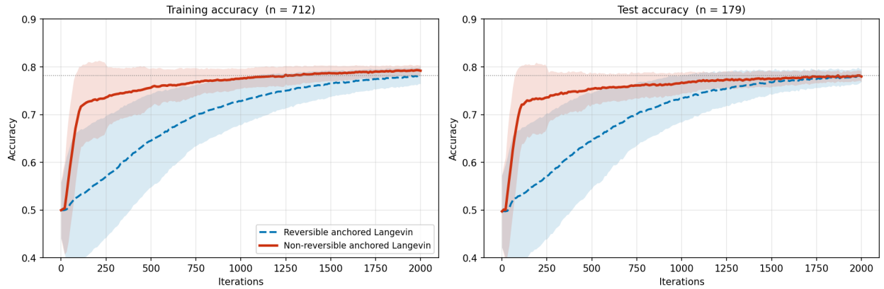
Figure 10: Accuracy over the training set and the test set for the Titanic dataset over smoothed l_1 ball. The red part (solid line) denotes the mean and standard deviation of the non-reversible anchored Langevin algorithm with J_g(x) ( \alpha = 1 ), the blue part (dashed line) denotes the mean and standard deviation of the reversible anchored Langevin algorithm ( \alpha = 0 ), and the grey dotted line is the test accuracy of the Bayesian logistic regression fit.
