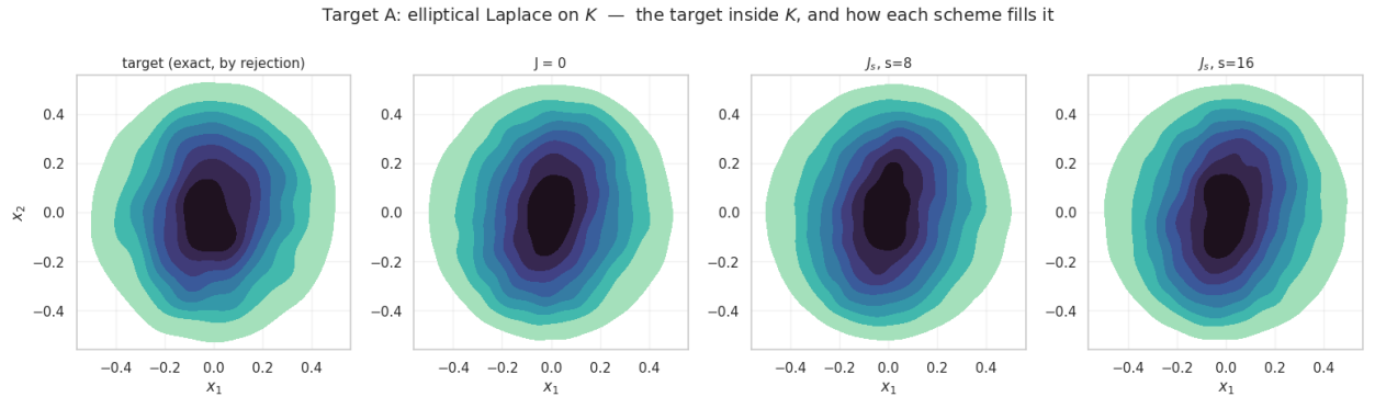
Figure 3: Visualized density plots of the first two coordinates (x_1, x_2) for target (A), U(x) = \|L^{-1}x\|_2 in (7.14), restricted to the ball K in (7.16). From left to right: 5000 exact samples of the target obtained by rejection, and the walkers of the reversible projected anchored Langevin algorithm ( J = 0 ) and of NRALD with J_s in (2.26) for s = 8 and s = 16 after 5000 iterates with \eta = 5 \times 10^{-4} (8 replicas of 5000 walkers), shown as kernel density estimates with the same contour levels.
