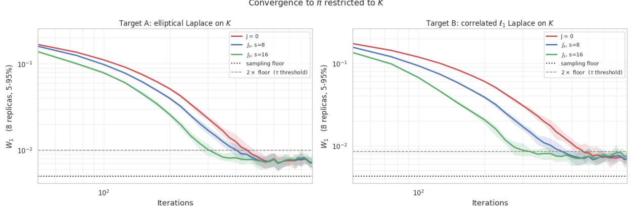
Figure 2: W_1 distance (7.20) between the walkers and an exact sample of the target, averaged over 8 replicas, as a function of the iterate on logarithmic axes, for the reversible projected anchored Langevin algorithm ( \alpha = 0 ) and NRALD with the tensor J_s in (2.26) with s = 8 and s = 16 ( \alpha = 1 ), for the targets (A) (7.14) (left) and (B) (7.15) (right) on the ball (7.16). The dotted line is the two-sample floor and the dashed line is 3 \times \text{floor} , the threshold of \tau_3 .
