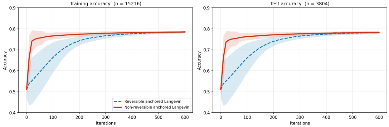
Figure 8: Accuracy over the training set and the test set for the Telescope dataset over the smoothed l_1 ball. The red part (solid line) denotes the mean and standard deviation of the non-reversible anchored Langevin algorithm with J_g(x) ( \alpha = 1 ), the blue part (dashed line) denotes the mean and standard deviation of the reversible anchored Langevin algorithm ( \alpha = 0 ), and the grey dotted line is the test accuracy of the Bayesian logistic regression fit.
