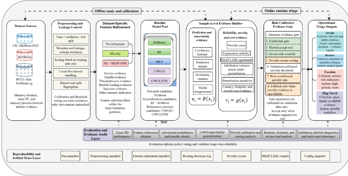
Fig. 1. EGAMA-RC study framework and runtime dataflow.
