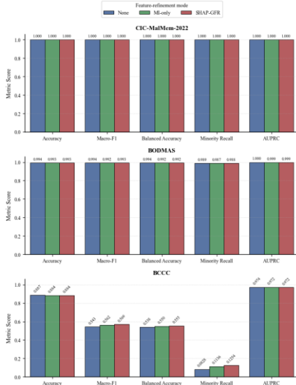
Fig. 2. Clean IID baseline performance under no refinement, MI-only refinement, and SHAP-GFR across CIC-MalMem-2022, BODMAS, and BCCC.
