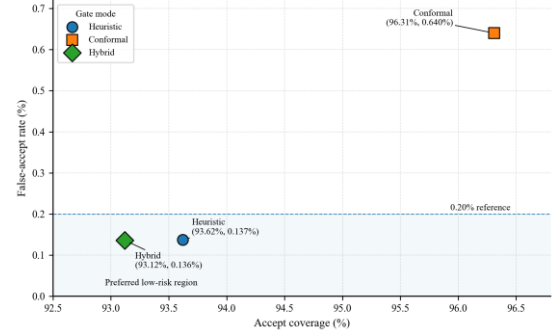
Fig. 3. Safety-throughput trade-off across EGAMA-RC gate configurations. Plot accept coverage on the x-axis and false-accept rate on the y-axis for heuristic, conformal, and hybrid gates.
