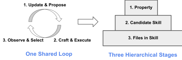
Figure 3: Architecture of Daydreaming
