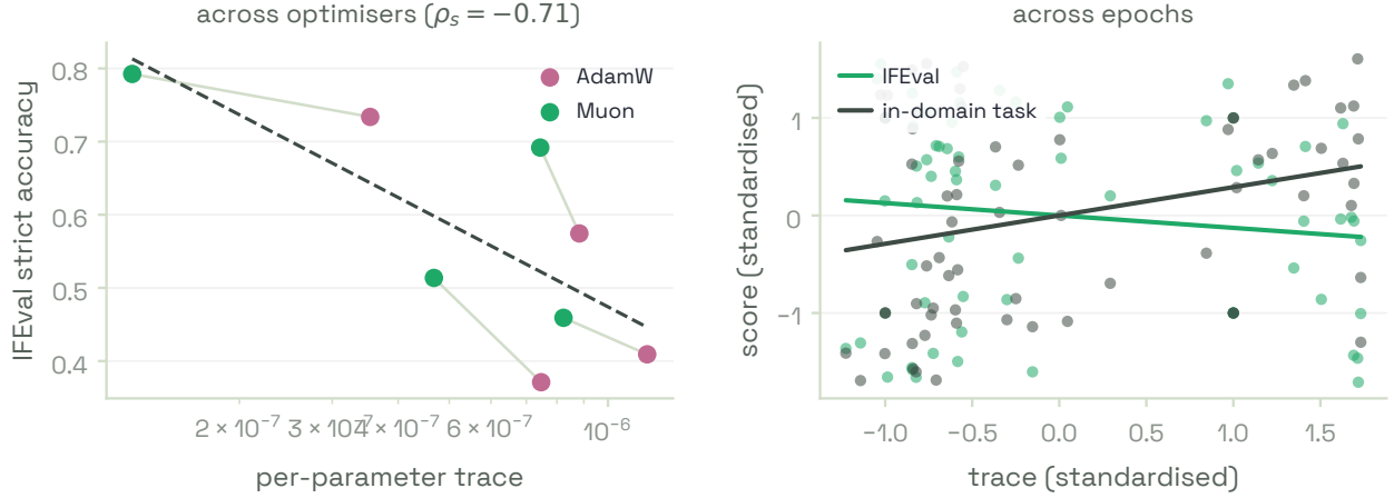
Figure 21: Flatness tracks retained general capability rather than in-domain quality. Left: across the eight validation-NLL-selected Muon (green) and AdamW (rose) checkpoints, IFEval rises as the per-parameter Fisher trace falls ( \rho_s = -0.71 ); each line joins a dataset’s pair, flatter and higher for Muon. Right: across the epoch sweep, standardised within (model, arm, dataset), a higher trace accompanies lower IFEval (green) but higher in-domain task score (graphite).
