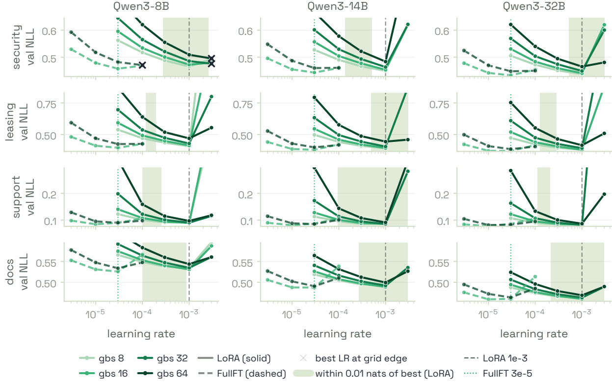
Figure 38: Learning-rate frontiers for the large Qwen3 sizes (8B, 14B, 32B), LoRA and FullIFT, faceted by dataset (rows) and model (columns).
