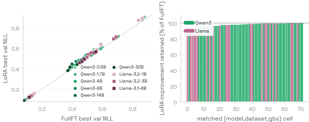
Figure 3: FullFT wins all 72 matched comparisons, but the margins are small. Left: paired best validation NLL at matched settings across all nine models (Qwen \bullet , Llama \blacksquare ). Right: the fraction of FullFT's improvement over baseline that LoRA recovers, coloured by family.
