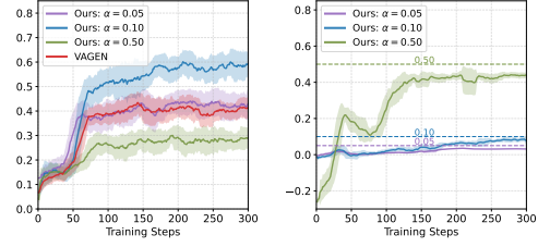
(a) Success Rate (b) Self-Consistency Reward
