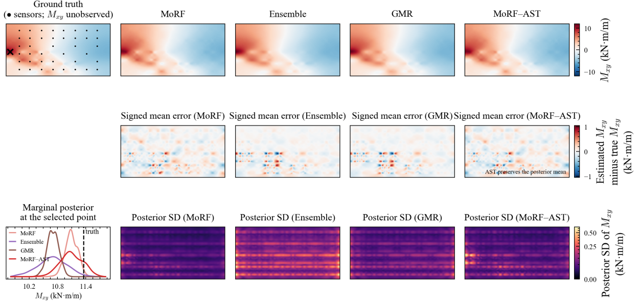
Figure 5: Full-field reconstruction and posterior spread under overload traffic
