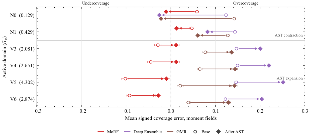
Figure 4: Signed coverage under active Bures transport
