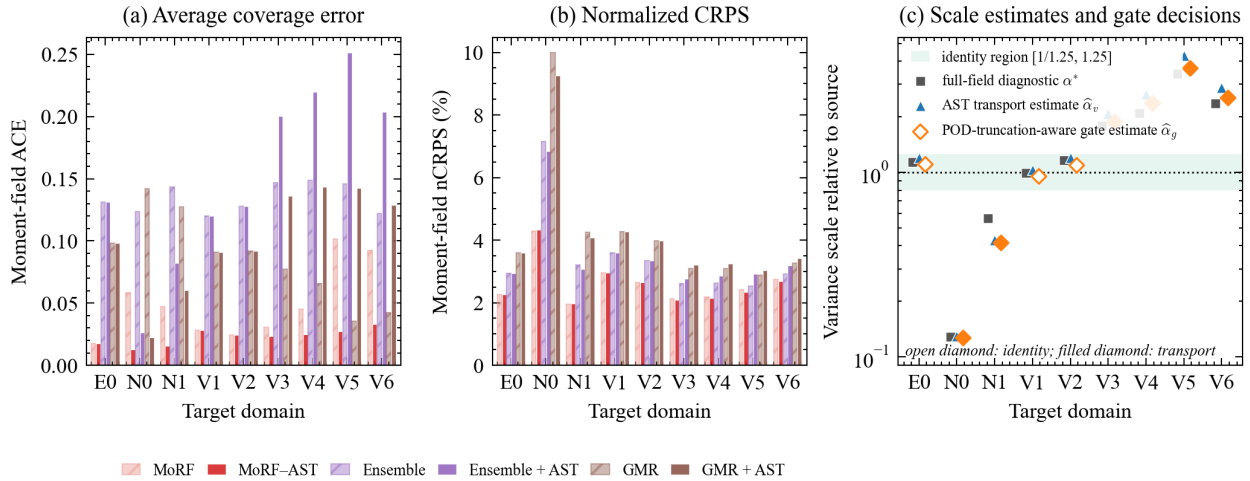
Figure 3: Cross-domain posterior calibration and AST routing
