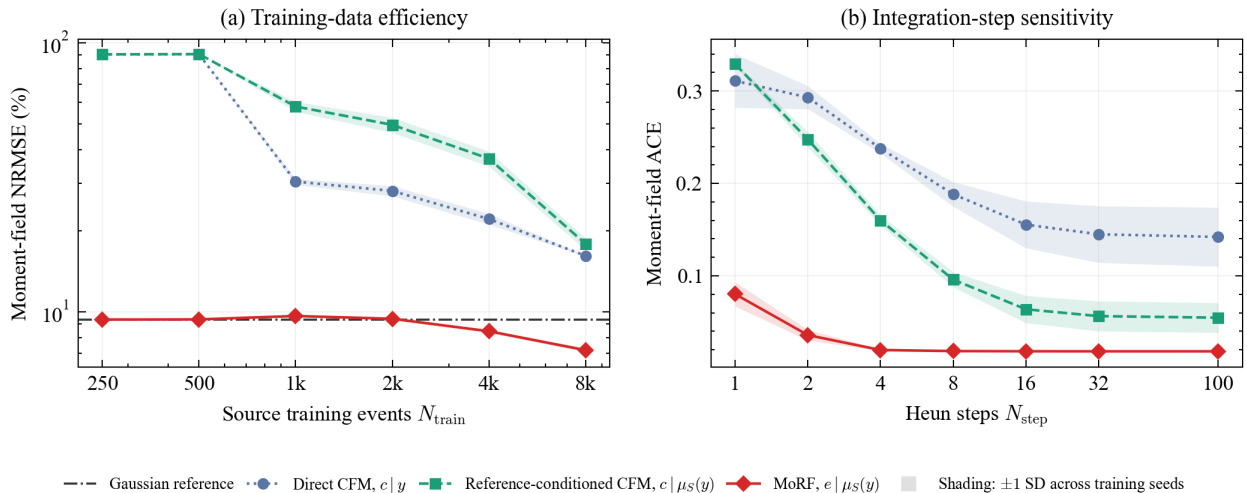
Figure 6: Training-data and integration-step sensitivity on the no-shift control
