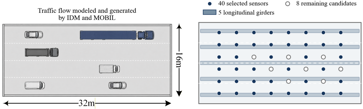
Figure 2: Bridge benchmark for probabilistic full-field reconstruction
