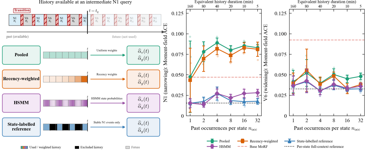
Figure 13: Context aggregation under recurrent operating states
