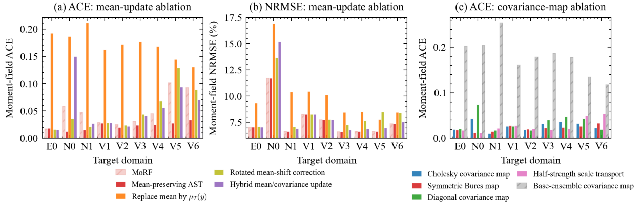
Figure 8: Posterior-center and covariance-map ablations across operational domains
