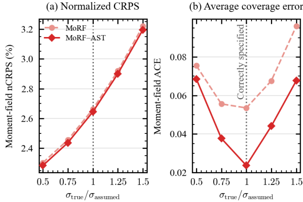
Figure 12: Observation-noise sensitivity of MoRF and MoRF-AST
